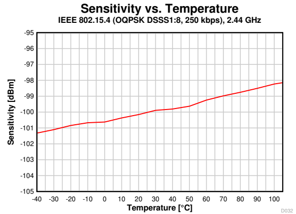
7-17. Sensitivity vs. Temperature (IEEE 802.15.4-2006, 250 kbps, OQPSK DSSS 1:8, 2.44GHz)
