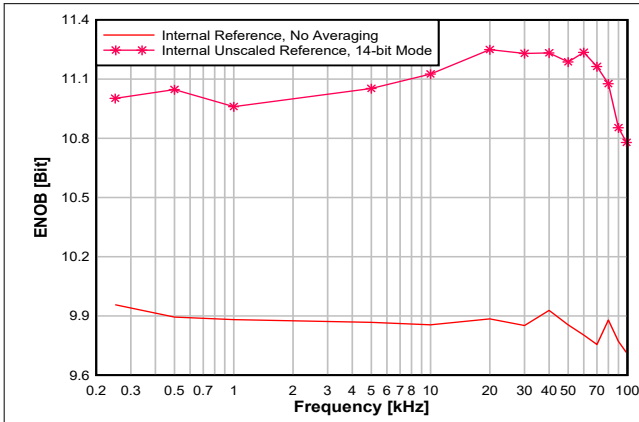
7-33. ENOB vs. Input Frequency
