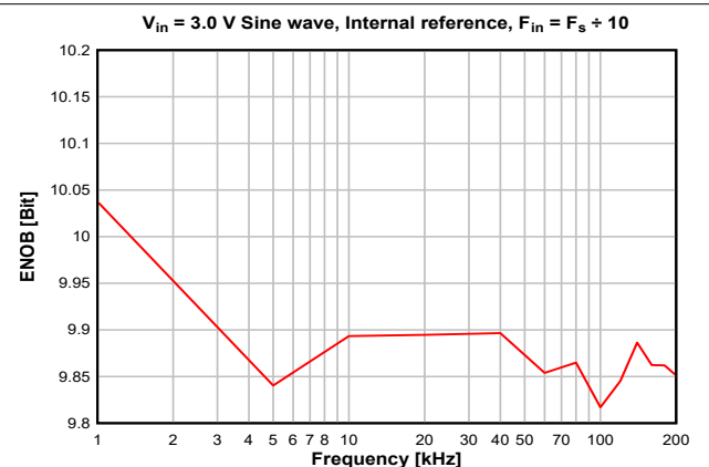
7-34. ENOB vs. Sampling Frequency
