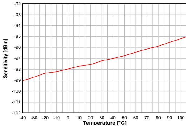
7-16. Sensitivity vs. Temperature (BLE 1Mbps, 2.44GHz)
