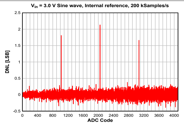
7-36. DNL vs. ADC Code
