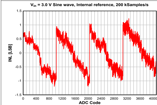
7-35. INL vs. ADC Code
