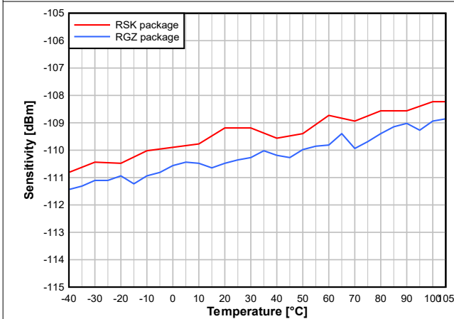
7-18. Sensitivity vs. Temperature (50kbps, 868.3MHz)
