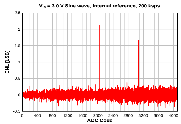
7-38. DNL vs. ADC Code
