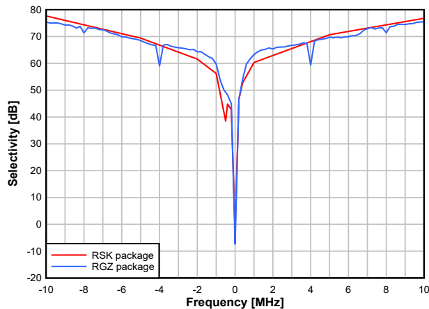
7-24. Selectivity vs. Frequency Offset (50kbps, 868.3MHz)
