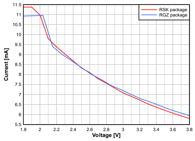
7-13. TX Current vs. Supply Voltage (VDDS) (BLE 1 Mbps, 2.44GHz, 0dBm)
