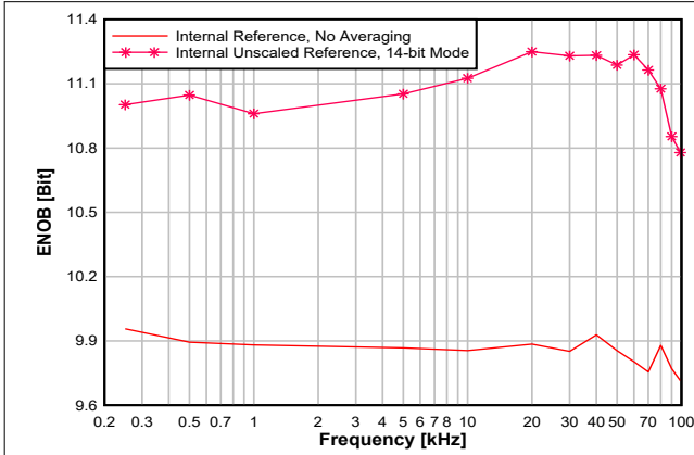
7-35. ENOB vs. Input Frequency
