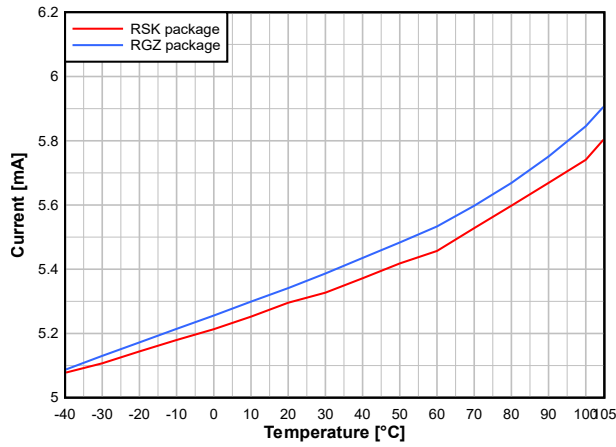
7-6. RX Current vs. Temperature (50kbps, 868.3MHz, VDD5 = 3.6V)
