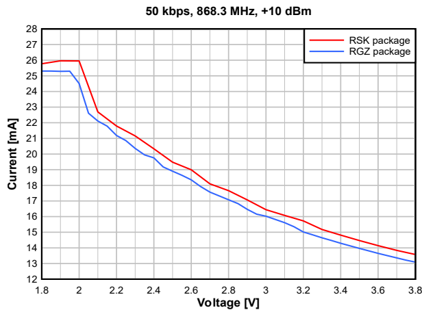
7-12. TX Current vs. Supply Voltage (VDDS) (50kbps, 868.3MHz)
