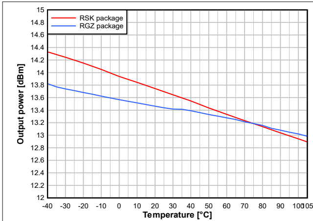
Figure 7-25. Output Power vs. Temperature (50kbps, 868.3MHz, +14dBm)
