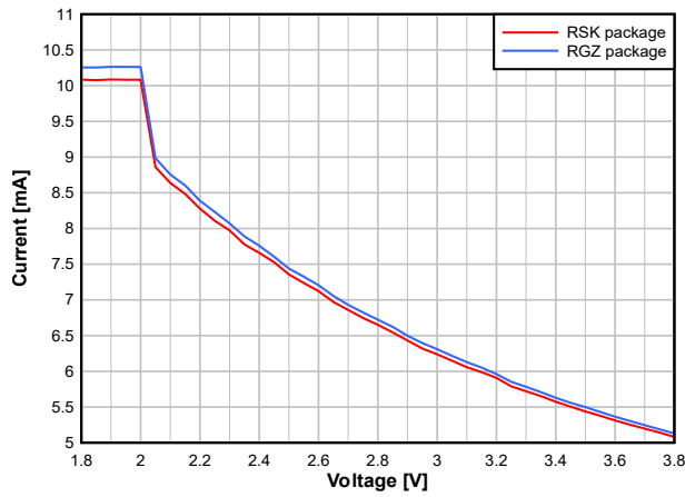
7-8. RX Current vs. Supply Voltage (VDD5) (50kbps, 868.3MHz)
