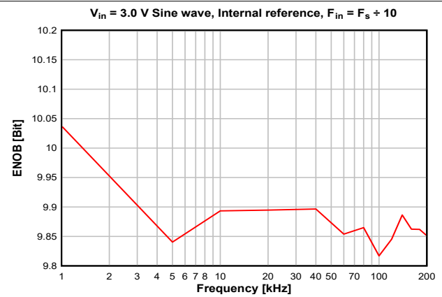
7-36. ENOB vs. Sampling Frequency
