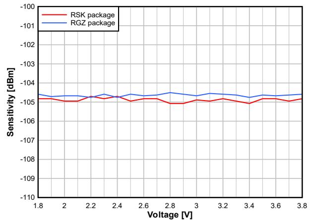
7-23. Sensitivity vs. Supply Voltage (VDD5) (250kbps, 2.44GHz)
