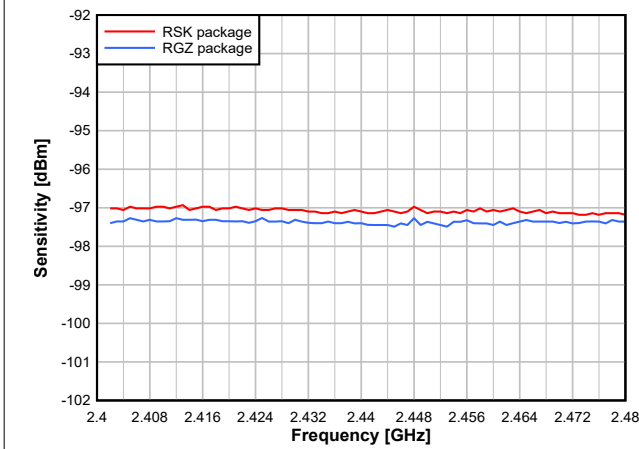
7-16. Sensitivity vs. Frequency (BLE 1Mbps, 2.44GHz)
