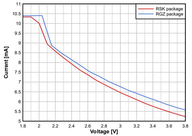
7-9. RX Current vs. Supply Voltage (VDD5) (BLE 1Mbps, 2.44GHz)
