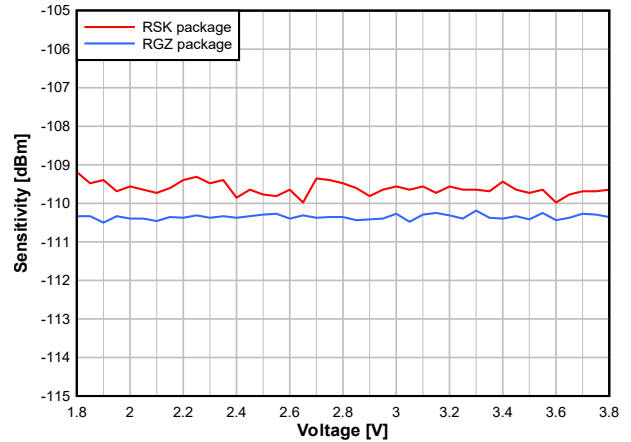
7-21. Sensitivity vs. Supply Voltage (VDD5) (50kbps, 868.3MHz)
