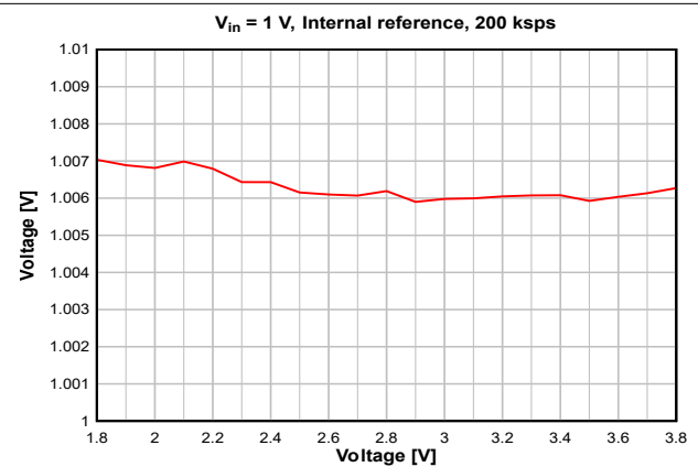
7-40. ADC Accuracy vs. Supply Voltage (VDD5)
