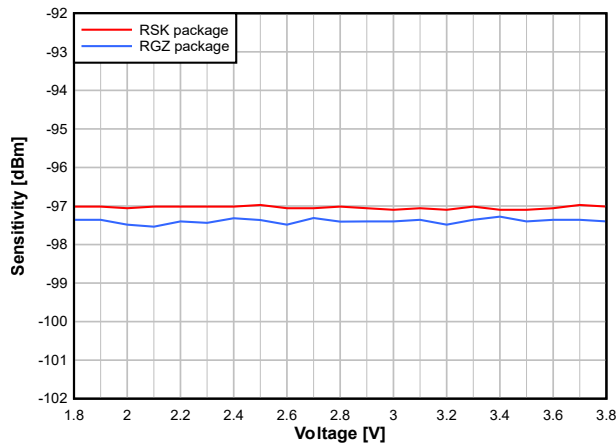
7-22. Sensitivity vs. Supply Voltage (VDD5) (BLE 1Mbps, 2.44GHz)
