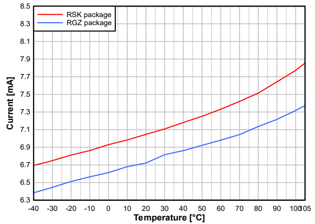
7-11. TX Current vs. Temperature (BLE 1Mbps, 2.44GHz, 0dBm)
