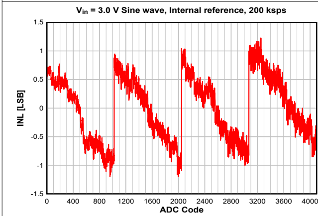
7-37. INL vs. ADC Code
