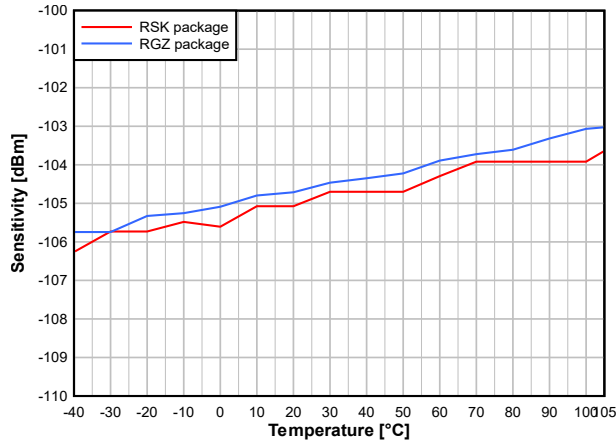
7-20. Sensitivity vs. Temperature (250kbps, 2.44GHz)
