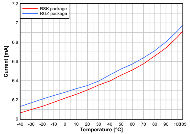
7-7. RX Current vs. Temperature (BLE 1Mbps, 2.44GHz)
