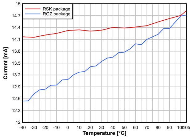
7-10. TX Current vs. Temperature (50kbps, 868.3MHz, +10dBm, VDDS = 3.6V)
