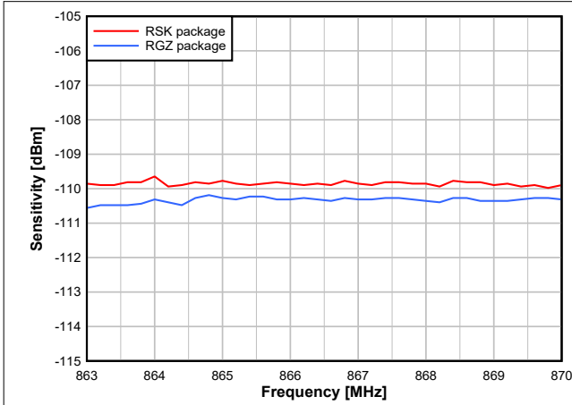
7-14. Sensitivity vs. Frequency (50kbps, 868MHz)
