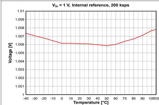
7-39. ADC Accuracy vs. Temperature
