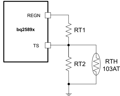
FIG 14. TS Resistor Network
