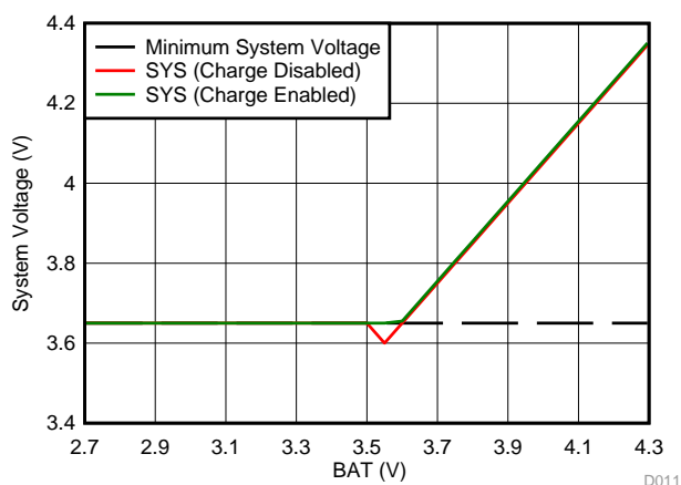
FIG 10. V(SYS) vs V(BAT)
