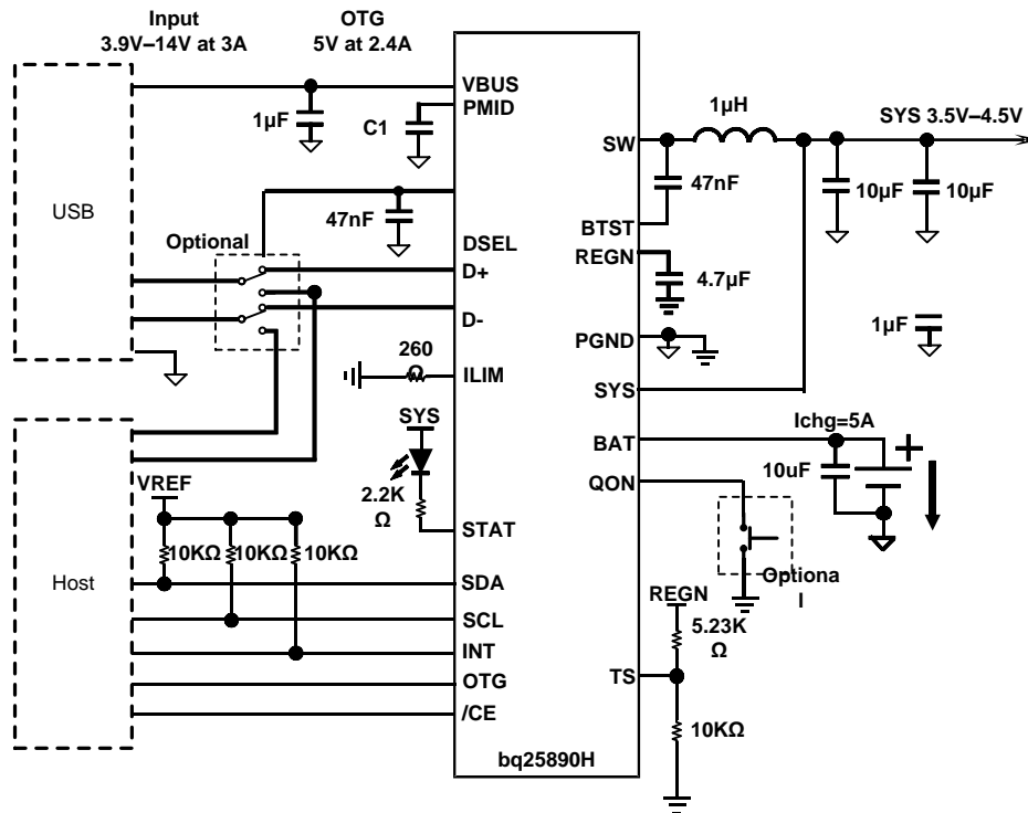
☒ 58. BQ25890H with D+/D- Interface, USB On-The-Go (OTG) and no Thermistor Connections
