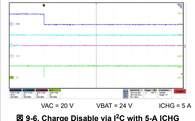
9-6. Charge Disable via I 2 C with 5-A ICHG
