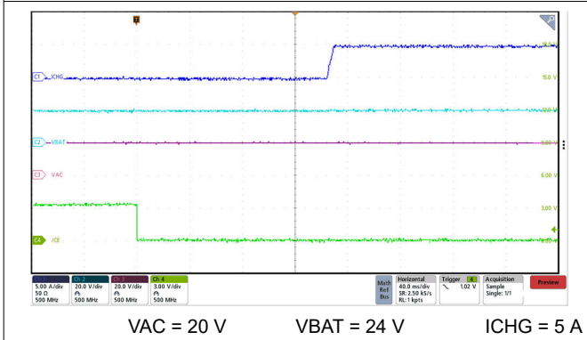
9-7. Charge Enable via CE Pin with 5-A ICHG
