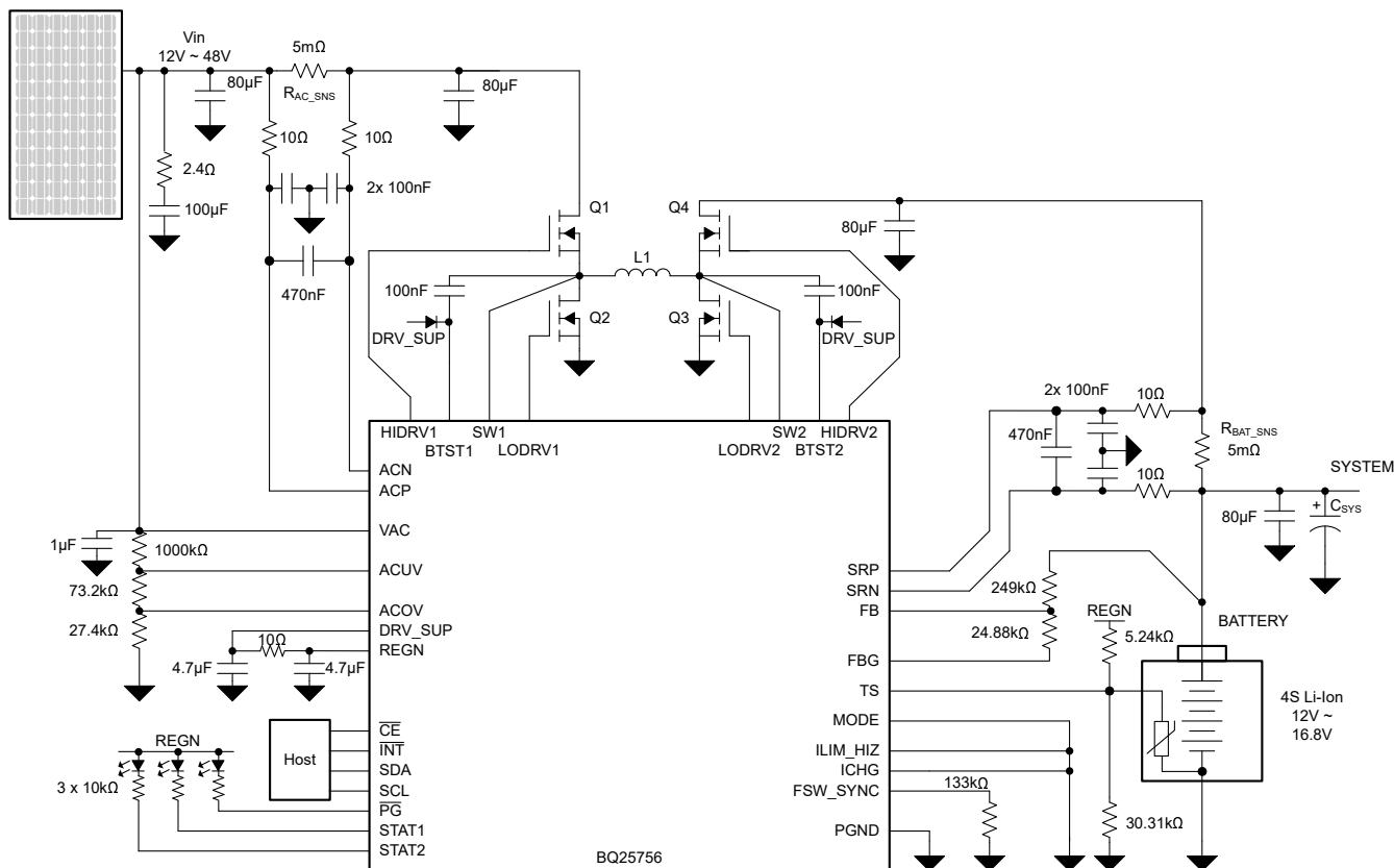
図 9-1. BQ25756: Solar Charging with Autonomous MPPT Algorithm to Charge 4s Battery with Maximum 15-A Charge Current
