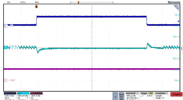
图 9-16. Reverse Mode Buck Transient Reponse
