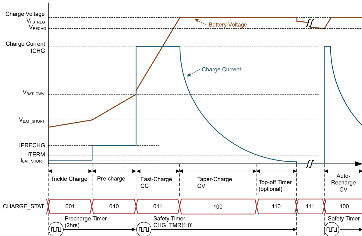
图 8-3. Typical Li-Ion Battery Charging Profile
