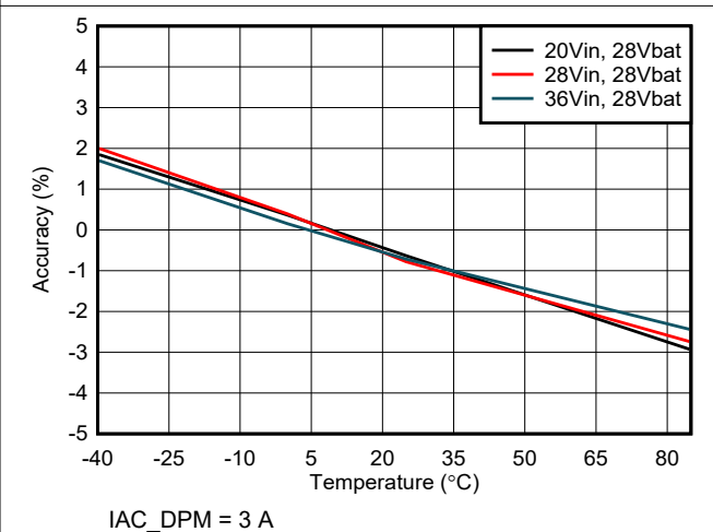
IAC_DPM = 3 A Figure 7-8. Input Current (IAC_DPM) Regulation Accuracy vs Temperature
