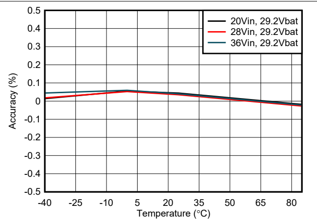
7-4. Charge Voltage Accuracy vs Temperature
