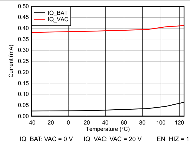
IQ_BAT: VAC = 0 V IQ_VAC: VAC = 20 V EN_HIZ = 1 Figure 7-6. Battery and Input Quiescent Current vs Temperature with VBAT = 28 V
