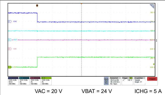
9-8. Charge Disable via CE Pin with 5-A ICHG
