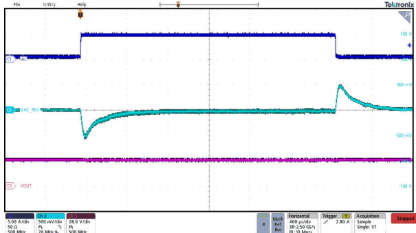
图 9-17. Reverse Mode Buck-Boost Transient Reponse
