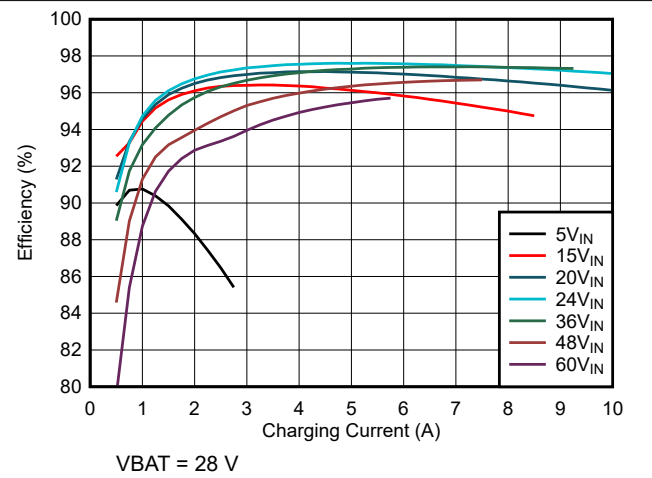
7-2. Charge Efficiency vs Charge Current (7s battery configuration)
