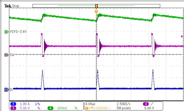
V_{VBUS} = 9\text{ V} I_{SYS} = 50\text{ mA} Charge Disabled 10-5. PFM Switching in Buck Mode
