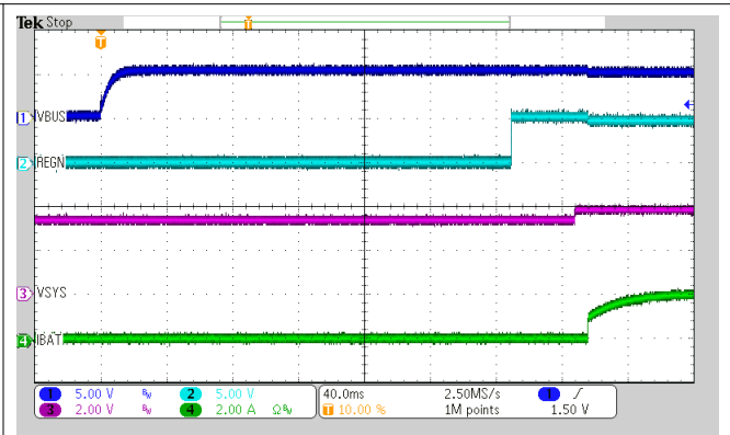
V_{VBUS} = 5\text{ V} V_{VBAT} = 3.2\text{ V} I_{CHG} = 2\text{ A} 10-3. Power-Up with Charge Enabled
