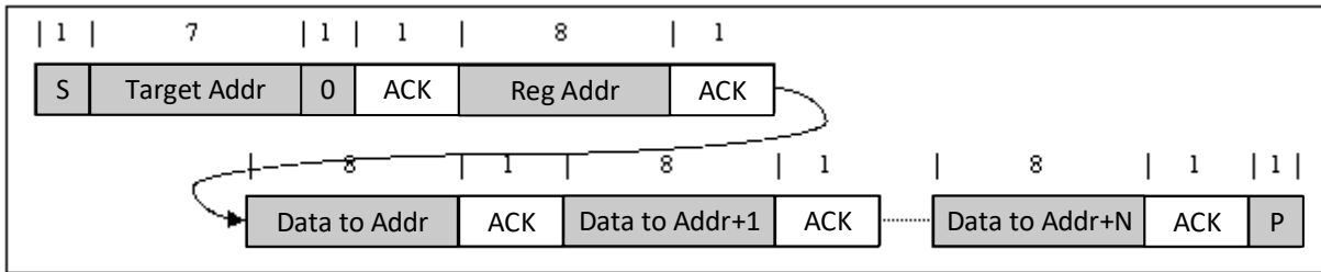
9-18. Multi-Write
