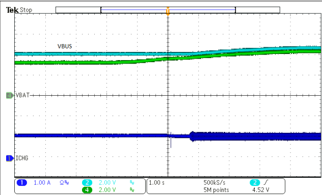
10-21. VINDPM Tracking Battery Voltage
