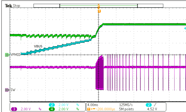
10-20. OTG Start-Up
