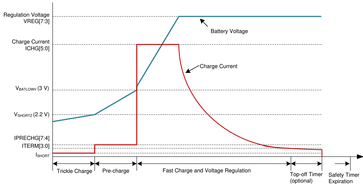
9-2. Battery Charging Profile
