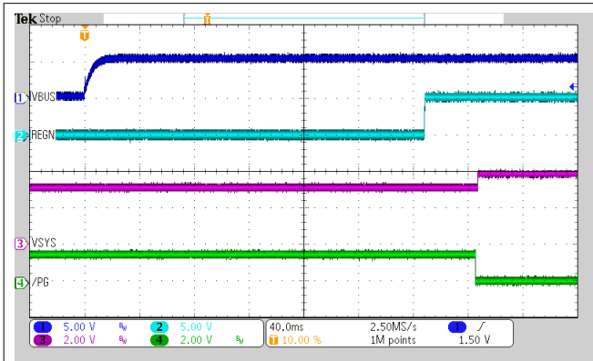
V_{VBUS} = 5\text{ V} V_{VBAT} = 3.2\text{ V} 10-2. Power-Up with Charge Disabled
