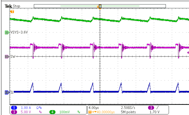
V_{VBUS} = 5\text{ V} I_{SYS} = 50\text{ mA} Charge Disabled 10-4. PFM Switching in Buck Mode
