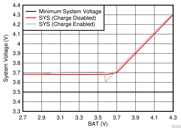
Figure 9-7. System Voltage vs Battery Voltage
