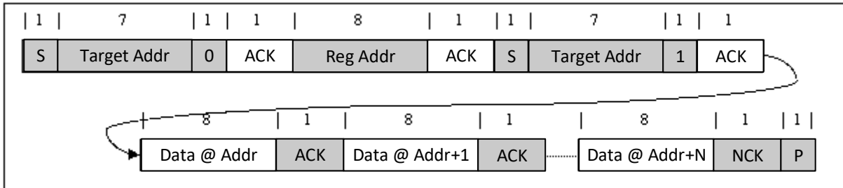
9-19. Multi-Read
