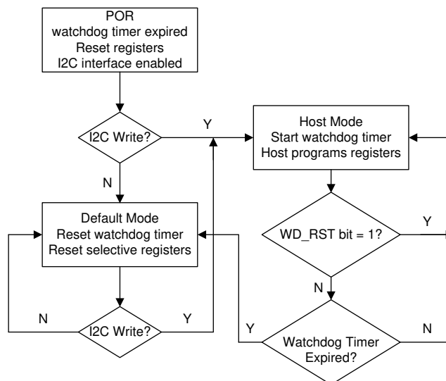
9-1. Watchdog Timer Flow Chart
