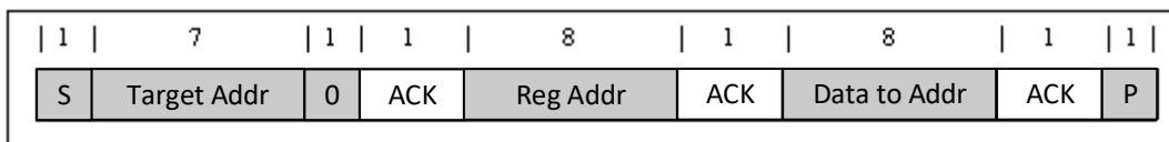
Figure 9-16. Single Write
