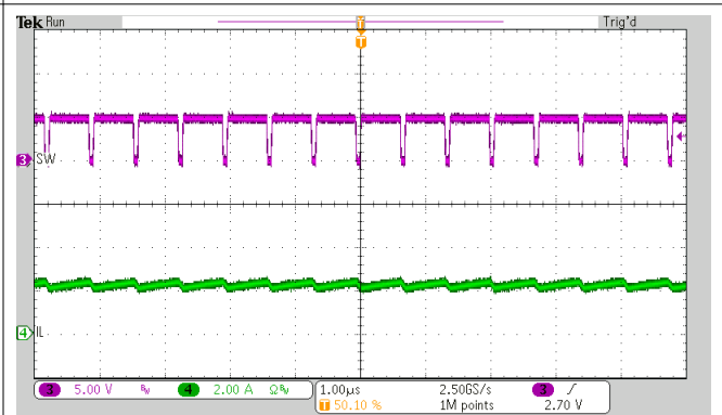
V_{VBUS} = 5\text{ V} V_{VBAT} = 3.8\text{ V} I_{CHG} = 2\text{ A} 10-7. PWM Switching in Buck Mode
