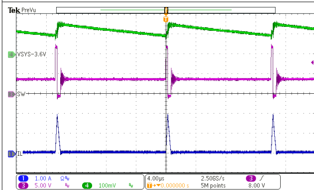
V_{VBUS} = 12\text{ V} I_{SYS} = 50\text{ mA} Charge Disabled 10-6. PFM Switching in Buck Mode
