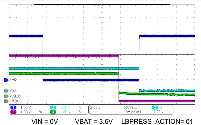
Figure 10-7. Ship Mode Entry with MR Long Button Press
