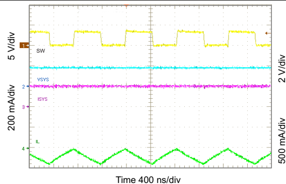
⊗ 65. Light Load Operation Showing SW
