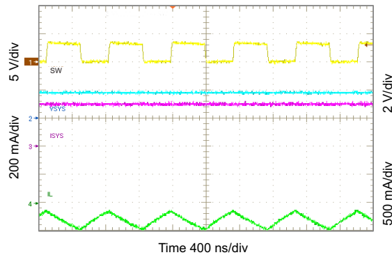
⊗ 66. Light Load Operation Showing SW
