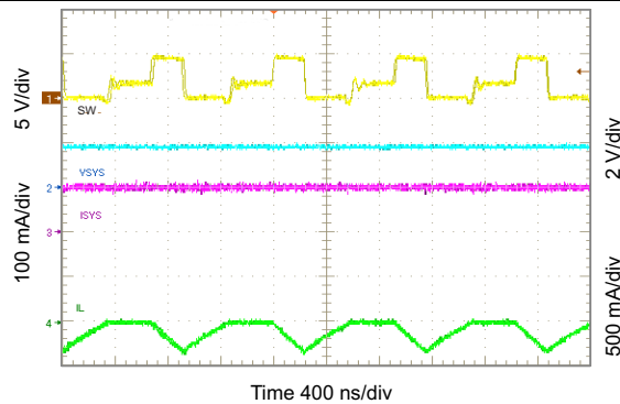
⊗ 64. Light Load Operation Showing SW
