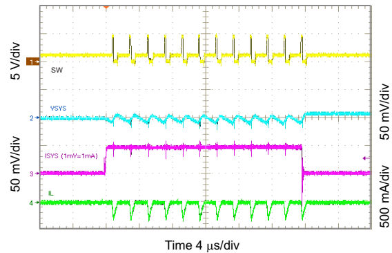
⊗ 67. Light Load Operation Showing SW
