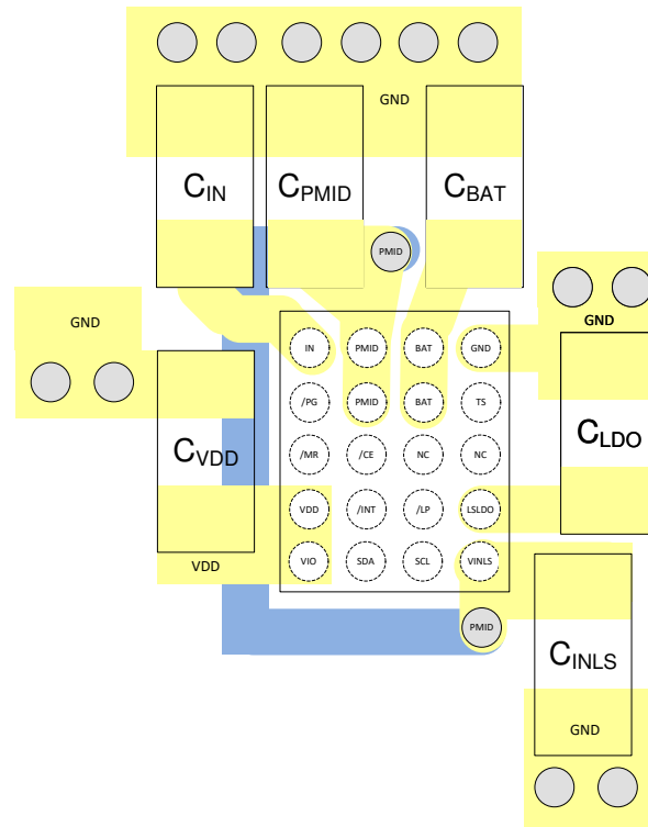
10-1. Layout Example
