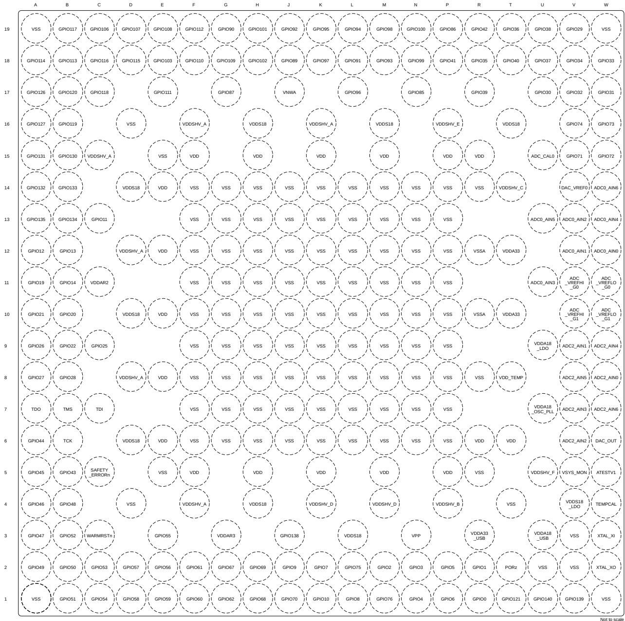
5-4. AM261x ZNC Pin Diagram
