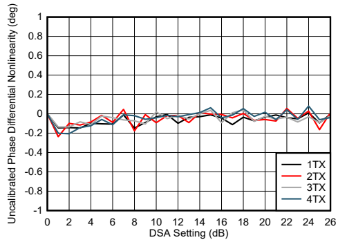
4-244. TX DSA Uncalibrated Phase Differential Nonlinearity
