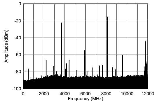
-12dBFS 4-207. TX Single Tone Output Spectrum at 8.1GHz
