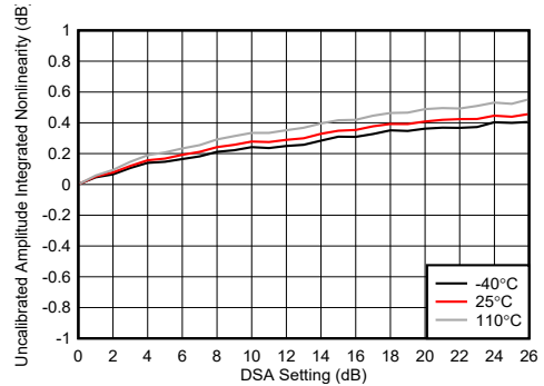
4-242. TX DSA Uncalibrated Amplitude Integrated Nonlinearity
