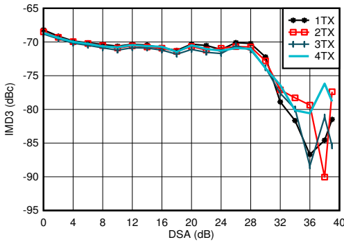
f_{DAC} = 11796.48\text{MSPS} , interleaved mode, matching at 4.9GHz, f_{CENTER} = 4.9\text{GHz} , -13\text{dBFS} each tone
