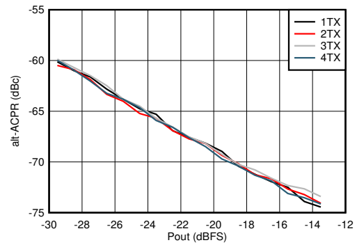
4-105. TX 20-MHz LTE alt-ACPR vs Digital Level at 2.6GHz
