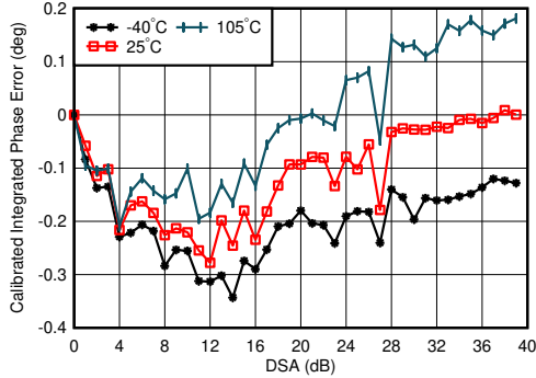
f_{DAC} = 11796.48\text{MSPS} , interleaved mode, matching at 4.9GHz, channel with the median variation over DSA setting at 25°C Integrated Phase Error = Phase(DSA Setting) – Phase(DSA Setting = 0)
