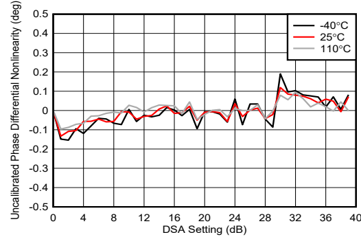
4-197. TX DSA Uncalibrated Phase Differential Nonlinearity at 8.1GHz
