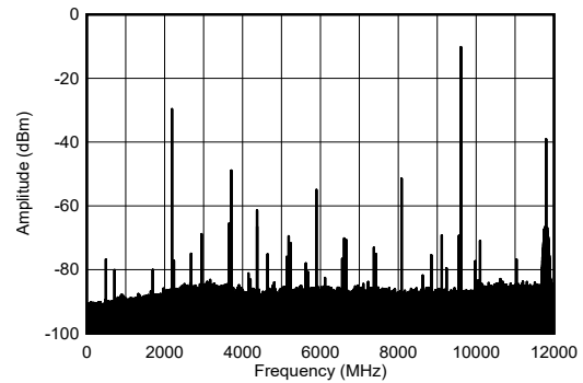
4-266. TX Single Tone Spectrum at 9.61GHz and -1dBFS (wideband)
