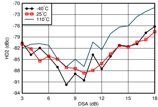
4-412. RX HD2 vs DSA and Temperature at 4.9GHz
