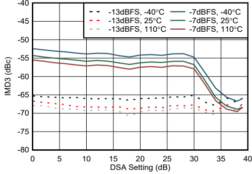
4-220. TX IMD3 vs DSA Setting at 8.11GHz
