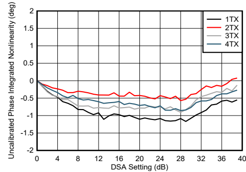
4-199. TX DSA Uncalibrated Phase Integrated Nonlinearity at 8.1GHz
