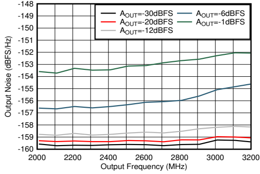
4-102. TX Single Tone Output Noise vs Frequency and Amplitude at 2.6GHz
