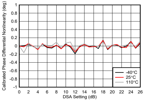
4-247. TX DSA Calibrated DSA Phase Differential Nonlinearity
