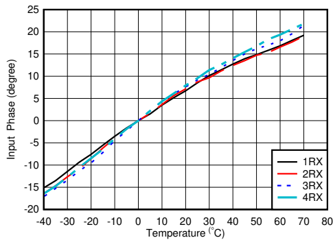
4-318. RX Input Phase vs Temperature and DSA at f_{IN} = 1.75\text{GHz}
