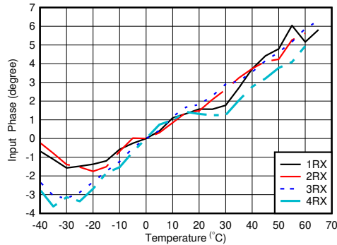
4-287. RX Input Phase vs Temperature and DSA at f_{OUT} = 0.8\text{GHz}
