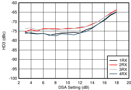
4-358. RX HD3 vs DSA Setting and Channel at 2.6GHz
