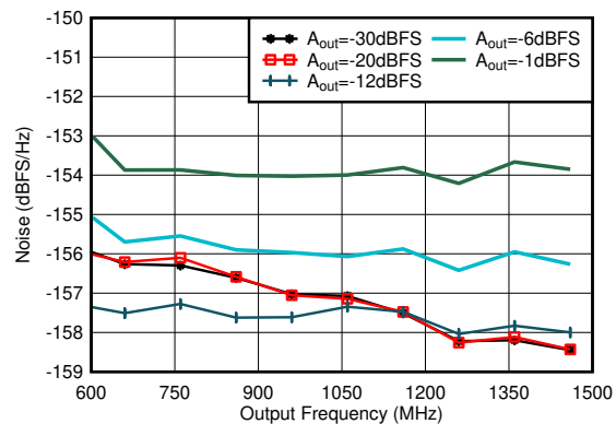
Matching at 2.6GHz, Single tone, f_{\text{DAC}} = 11.79648\text{GSPS} , interleave mode, 40MHz offset, DSA = 0dB
