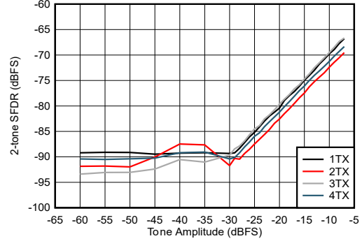
4-221. TX 2-Tone SFDR vs Digital Amplitude at 8.11GHz
