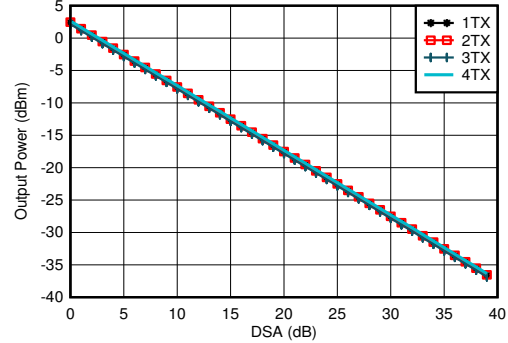
f_{\text{DAC}} = 8847.36\text{MSPS} , A_{\text{out}} = -0.5\text{dBFS} , matching 2.6GHz
