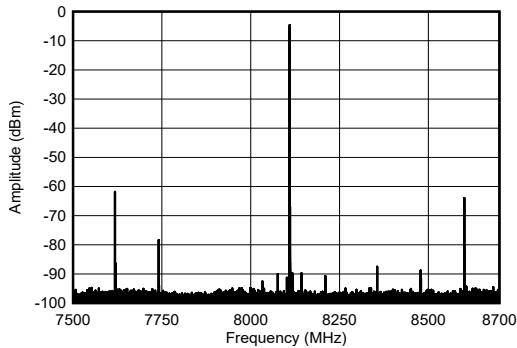
-1dBFS 4-204. TX Single Tone Output Spectrum at 8.1GHz
