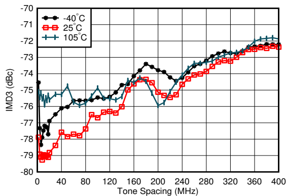
f_{DAC} = 5898.24\text{MSPS} , straight mode, f_{CENTER} = 0.85\text{GHz} , matching at 0.8GHz, -13\text{dBFS} each tone, worst channel
