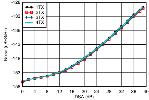
f_{DAC} = 11796.48\text{MSPS} , interleaved mode, matching at 4.9GHz, P_{OUT} = -13\text{dBFS}
