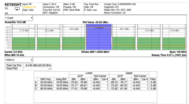
4-103. TX 20-MHz LTE Output Spectrum at 2.6GHz (Band 41)
