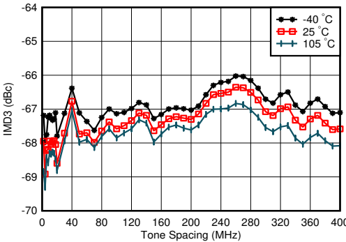
f_{DAC} = 11796.48\text{MSPS} , interleaved mode, matching at 4.9GHz, f_{CENTER} = 4.9\text{GHz} , -13\text{dBFS} each tone, worst channel
