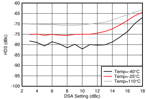
4-359. RX HD3 vs DSA Setting and Temperature at 2.6GHz
