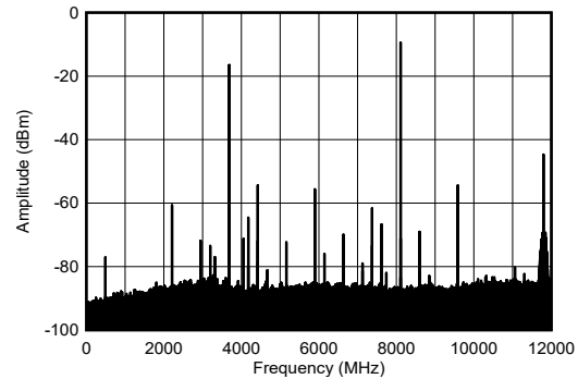
-6dBFS 4-205. TX Single Tone Output Spectrum at 8.1GHz
