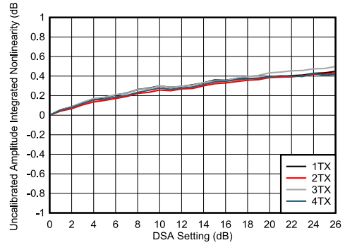
4-240. TX DSA Uncalibrated Amplitude Integrated Nonlinearity
