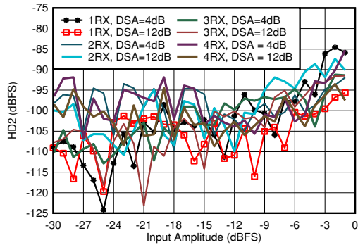
4-334. RX HD2 vs DSA Setting and Channel at 1.9 GHz
