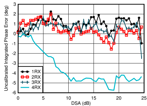
4-400. RX Uncalibrated Differential Phase Error vs DSA Setting at 4.9GHz
