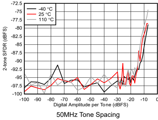
图 4-440. RX 2-tone SFDR vs Digital Amplitude at 8.11GHz
