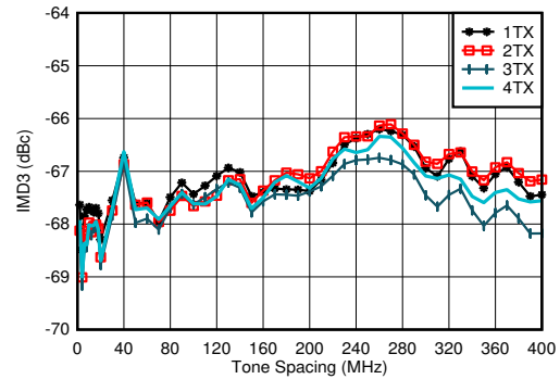
f_{DAC} = 11796.48\text{MSPS} , interleaved mode, matching at 4.9GHz, f_{CENTER} = 4.9\text{GHz} , -13\text{dBFS} each tone
