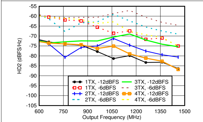
Matching at 0.8GHz, f_{DAC} = 5898.2\text{GSPS} , straight mode
