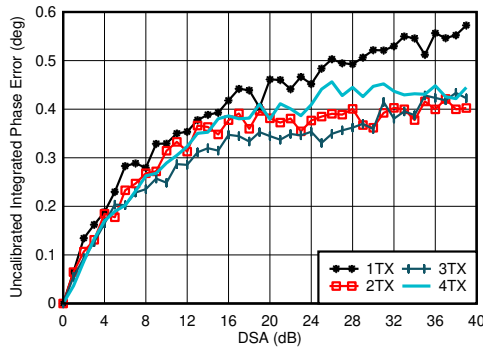
Figure 4-126. TX Uncalibrated Integrated Phase Error vs DSA Setting and Channel at 3.5GHz
