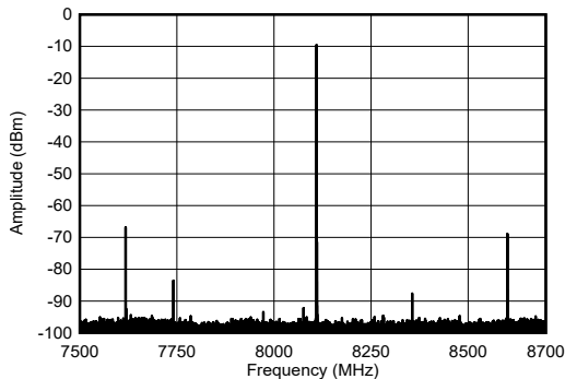
-6dBFS 4-206. TX Single Tone Output Spectrum at 8.1GHz
