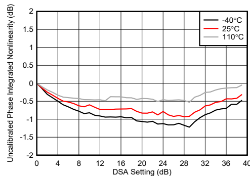
4-201. TX DSA Uncalibrated Phase Integrated Nonlinearity at 8.1GHz
