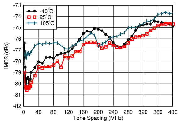
DAC = 8847.3\text{MSPS} , straight mode, f_{CENTER} = 0.85\text{GHz} , matching at 0.8 GHz, -13\text{dBFS} each tone, worst channel
