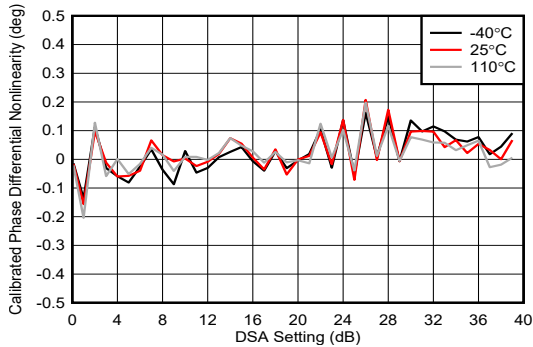
4-198. TX DSA Calibrated Phase Differential Nonlinearity at 8.1GHz
