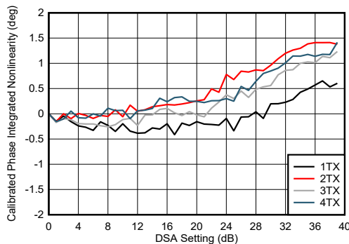
4-200. TX DSA Calibrated Phase Integrated Nonlinearity at 8.1GHz
