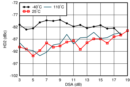
4-335. RX HD2 vs DSA Setting and Temperature at 1.9 GHz
