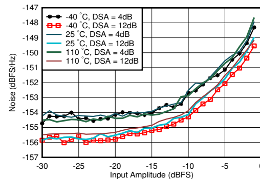
图 4-298. RX Noise Spectral Density vs Input Amplitude and Temperature at 0.8GHz
