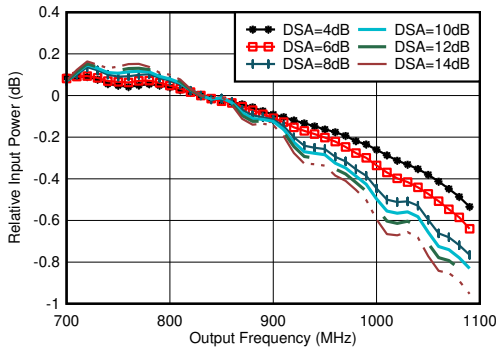
4-285. RX In-Band Gain Flatness for Channel 1RX, f_{IN} = 830\text{MHz}
