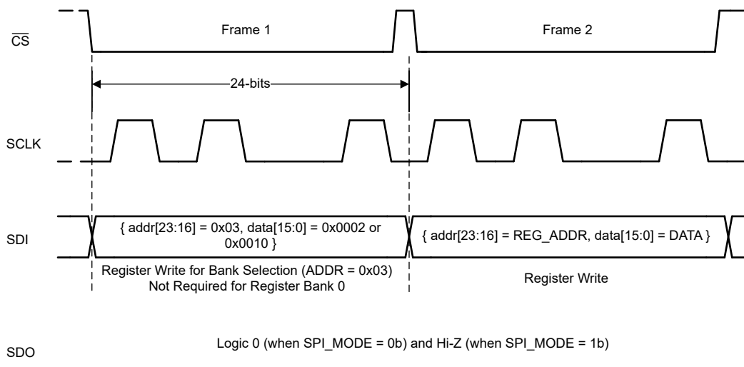
Figure 6-9. Register Write
