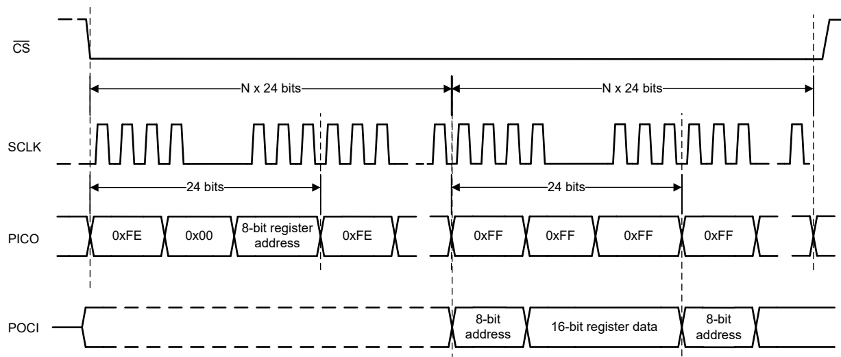
图 6-14. Register Read With Daisy-Chain Configuration
