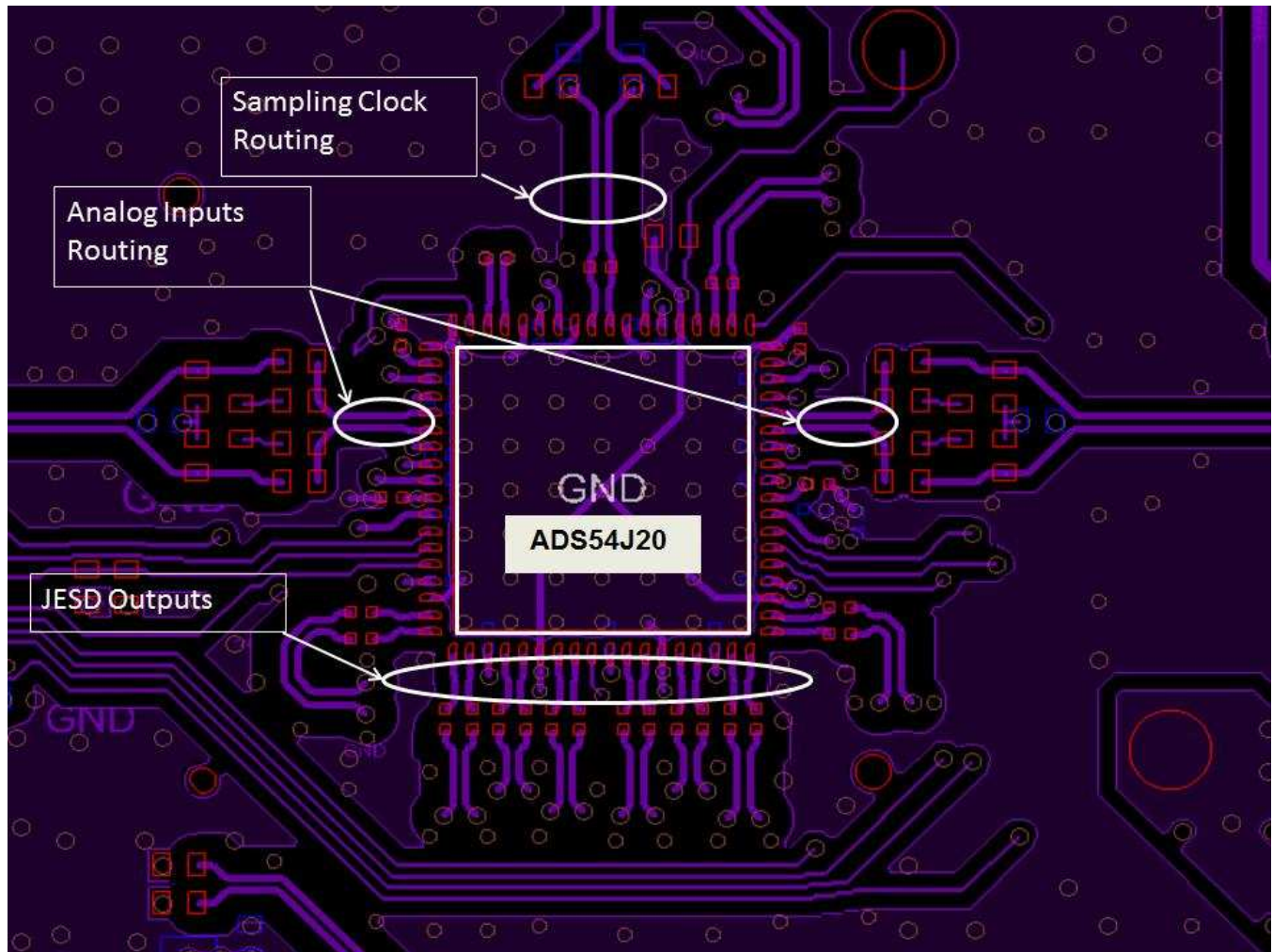
Figure 140. ADS54J20EVM Layout
