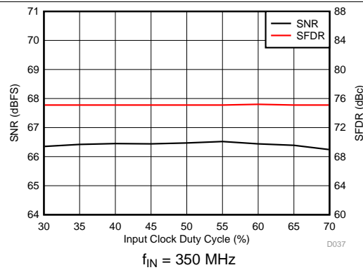
Figure 42. Performance vs Clock Duty Cycle
