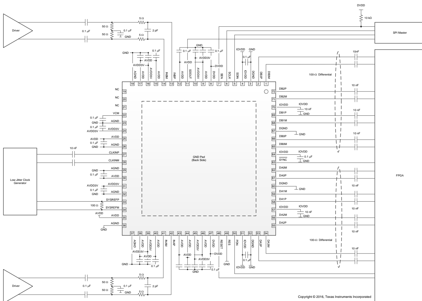
Figure 134. AC-Coupled Receiver
