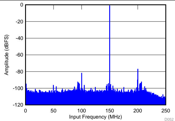
Figure 52. FFT for 450-MHz Input Signal in Decimate-by-4 Mode
