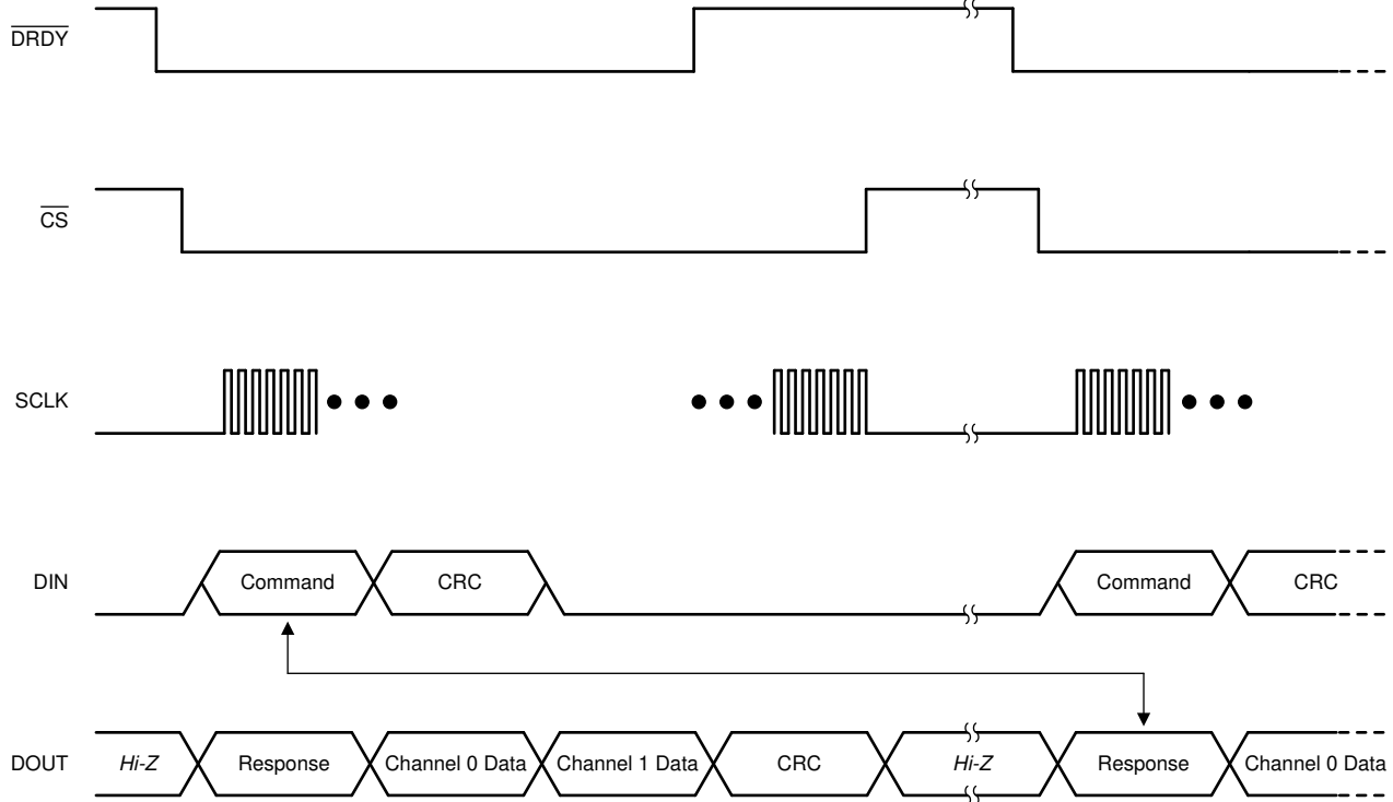
8-18. Typical Communication Frame
