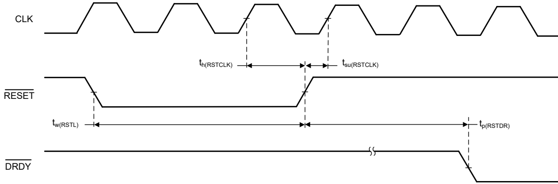
6-5. RESET Timing Requirements and Switching Characteristics
