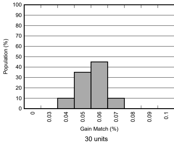
6-45. Gain Match Distribution
