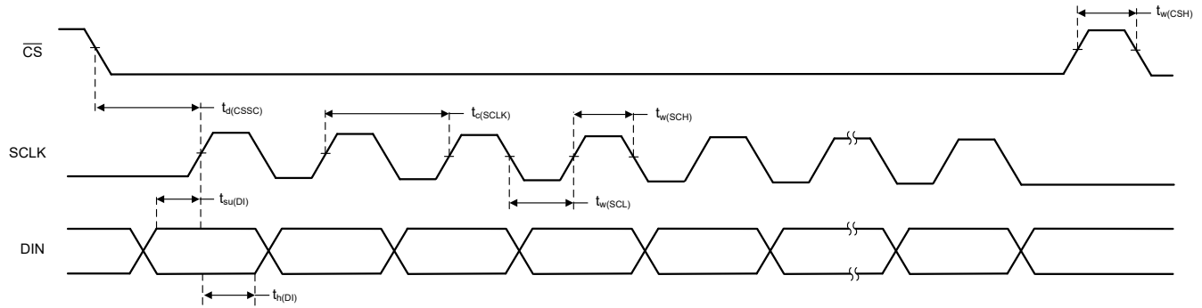
6-2. Serial Interface Timing Requirements
