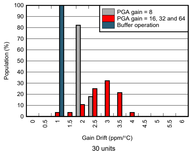
6-44. Gain Drift Distribution
