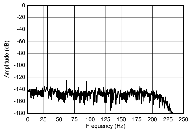
6-30. Low-Power Mode FFT Spectrum
