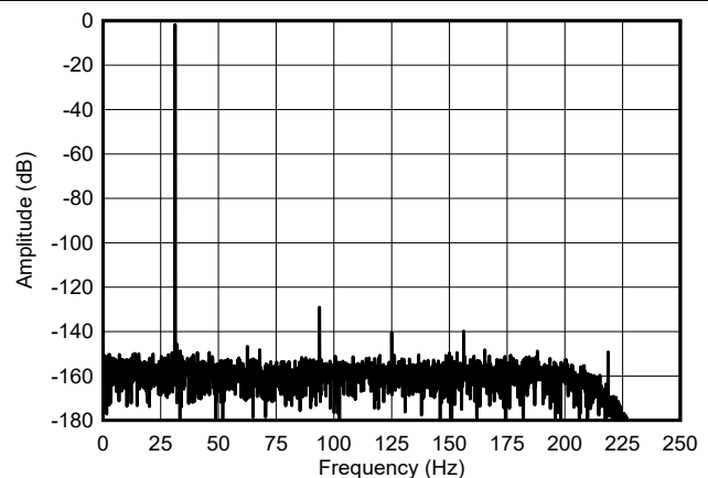
6-28. Low-Power Mode FFT Spectrum
