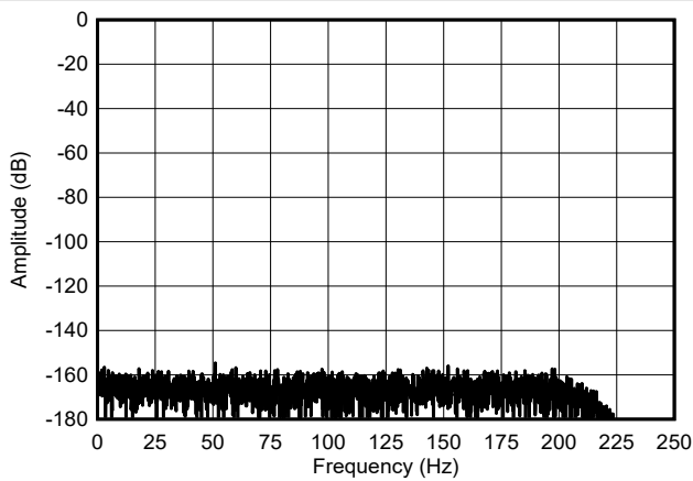
6-27. Low-Power Mode FFT Spectrum
