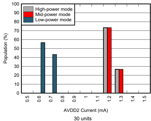
6-64. AVDD2 Current Distribution
