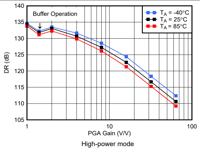
6-36. Dynamic Range vs PGA Gain
