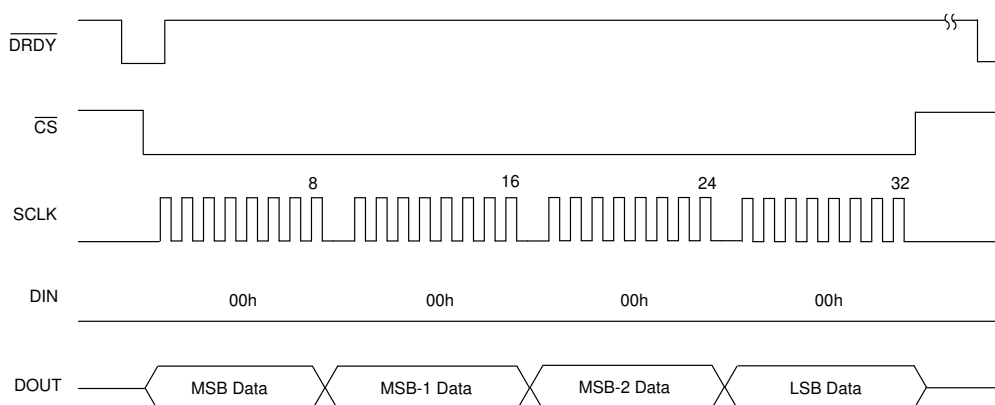
Figure 8-24. Read Data Direct
