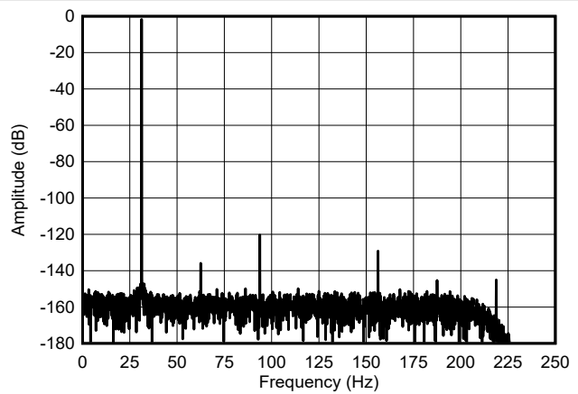
6-22. Mid-Power Mode FFT Spectrum
