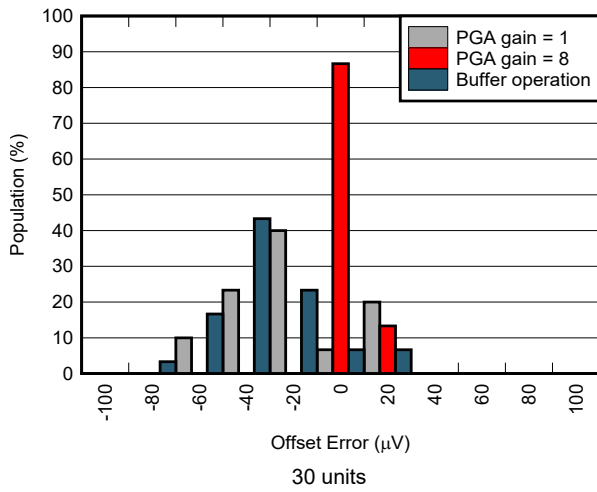
6-39. Offset Error Distribution
