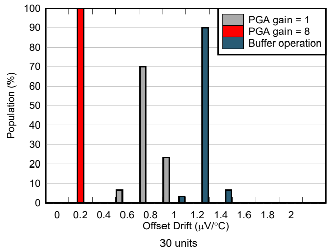
6-40. Offset Drift Distribution
