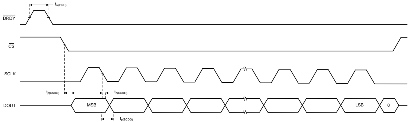
6-3. Serial Interface Switching Characteristics
