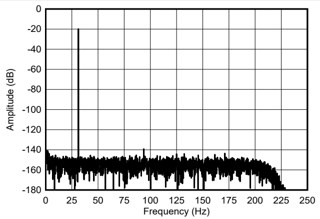
6-34. Low-Power Mode FFT Spectrum
