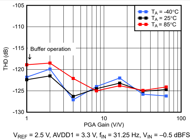
6-47. Mid-Power Mode THD vs PGA Gain
