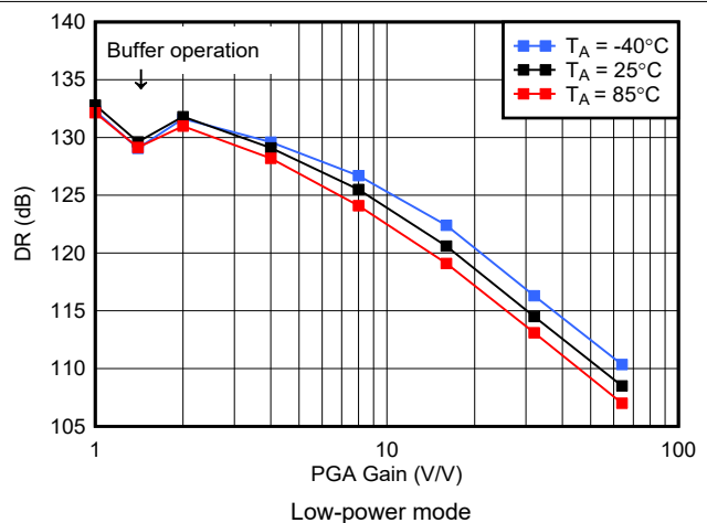
6-38. Dynamic Range vs PGA Gain
