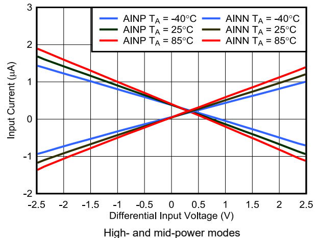
6-54. PGA Input Current vs Input Voltage
