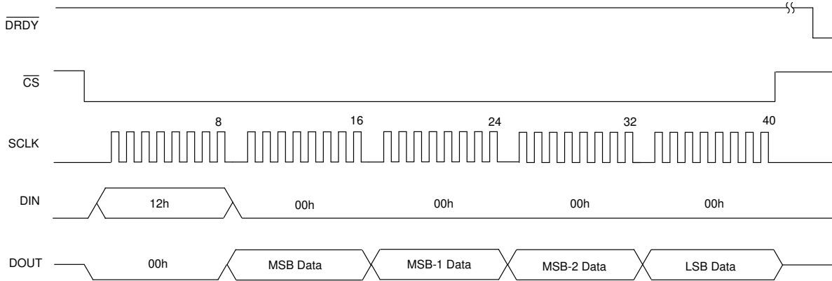
8-25. Read Conversion Data by Command
