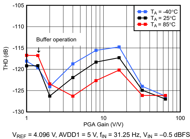
6-49. High-Power Mode THD vs PGA Gain
