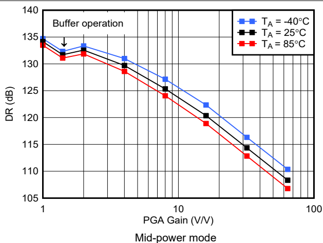
6-37. Dynamic Range vs PGA Gain
