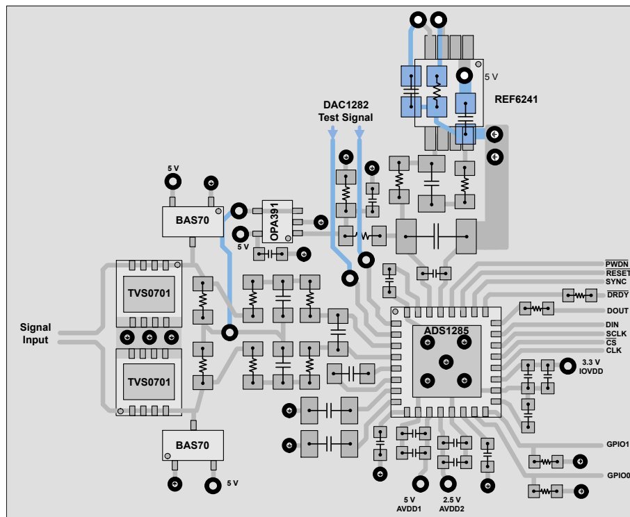
Figure 9-3. Example Layout
