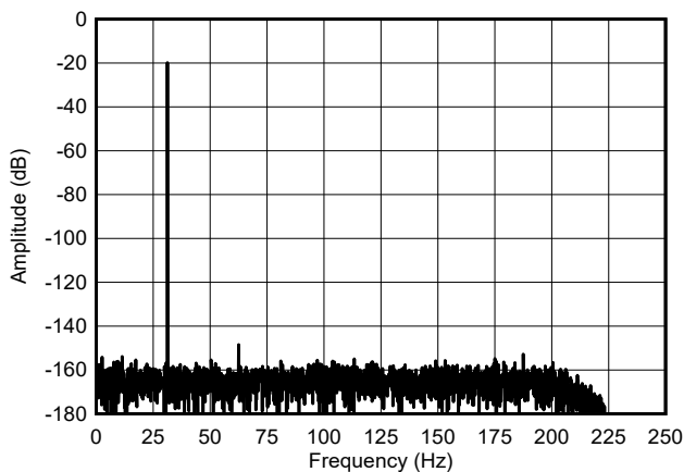
6-29. Low-Power Mode FFT Spectrum
