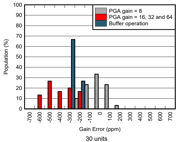
6-42. Gain Error Distribution
