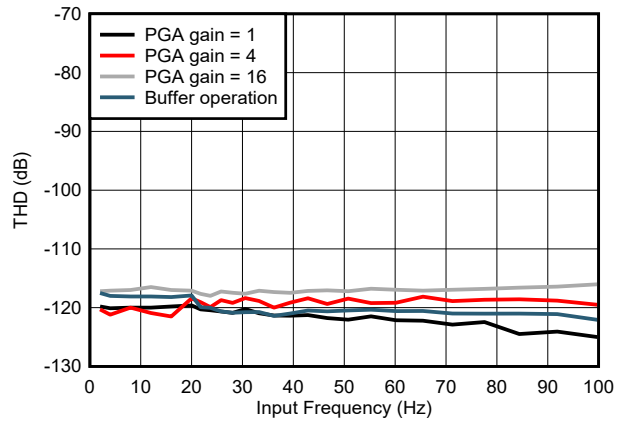
6-52. High- and Mid-Power Mode THD vs Input Frequency
