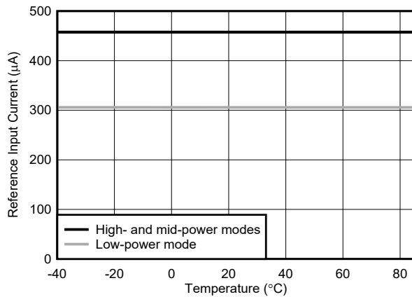
6-57. Reference Input Current vs Temperature
