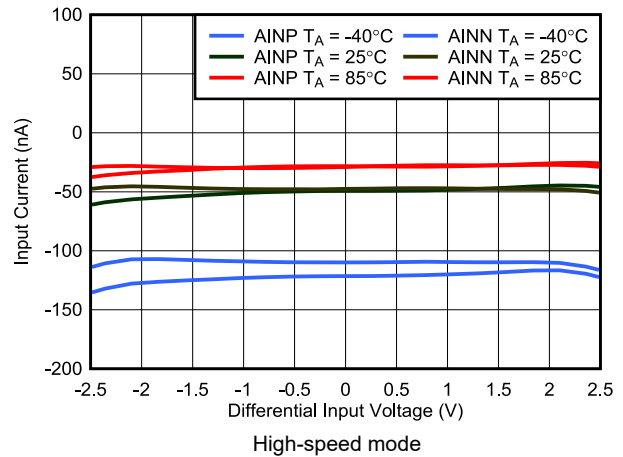
6-54. PGA Input Current vs Input Voltage
