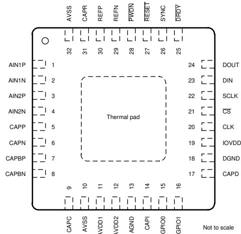
图 5-1. RHB Package, 32-Pin, 5-mm × 5-mm VQFN (Top View)
