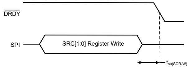
6-7. Sample Rate Converter Register-Write Timing Requirements
