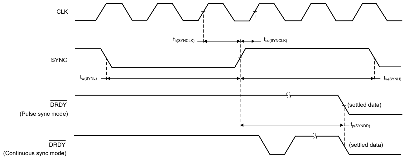
6-4. SYNC Timing Requirements and Switching Characteristics
