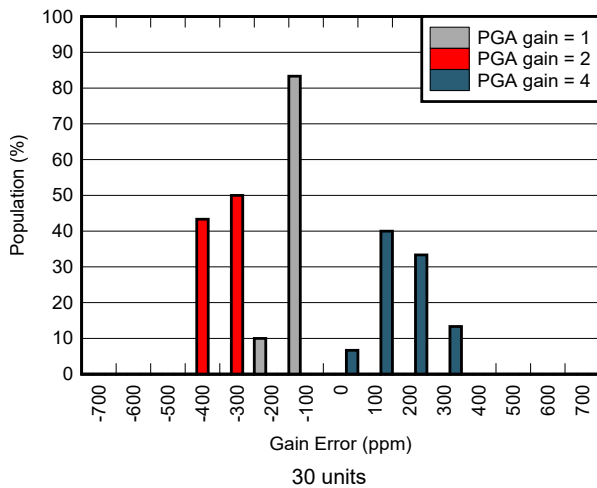
6-41. Gain Error Distribution
