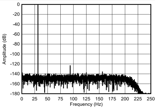
6-33. Low-Power Mode FFT Spectrum
