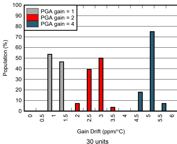
6-43. Gain Drift Distribution
