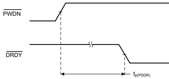
6-6. PWDN Switching Characteristics
