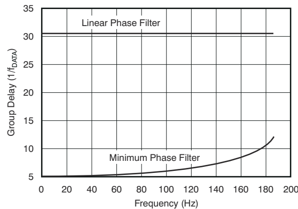
8-18. FIR Group Delay (f DATA = 500 SPS)
