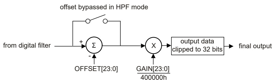
Figure 8-20. Calibration Block Diagram
