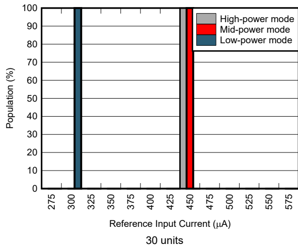
6-58. Reference Input Current Distribution
