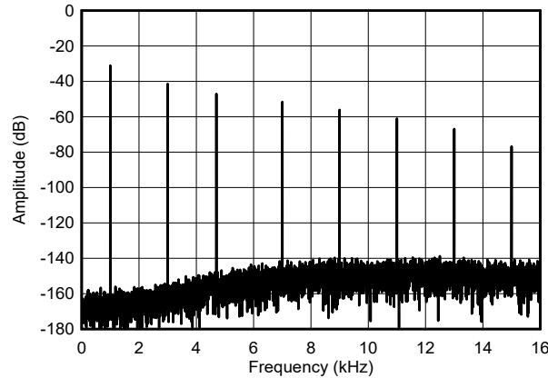
图 8-13. FFT Output of the Sinc Filter ( f_{DATA} = 32 kSPS)
