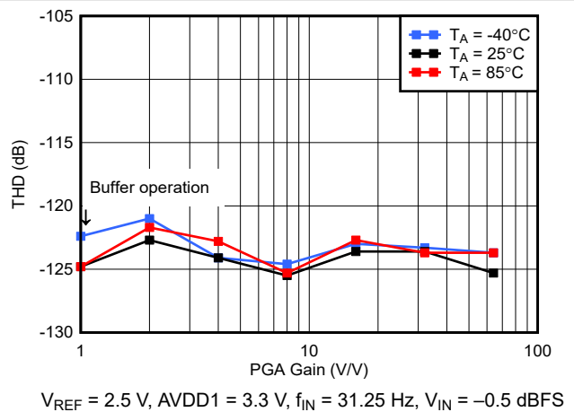
6-48. Low-Power Mode THD vs PGA Gain
