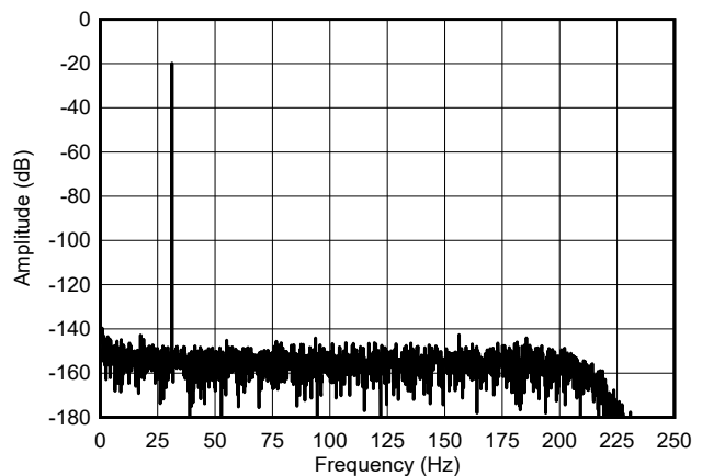
6-24. Mid-Power Mode FFT Spectrum
