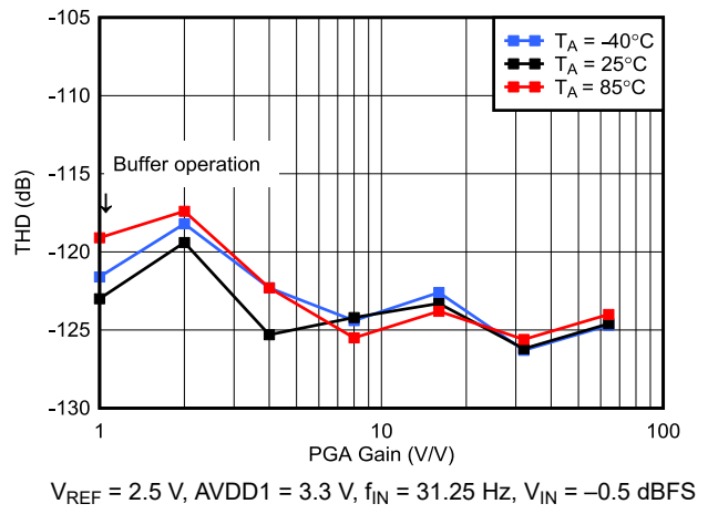
6-46. High-Power Mode THD vs PGA Gain
