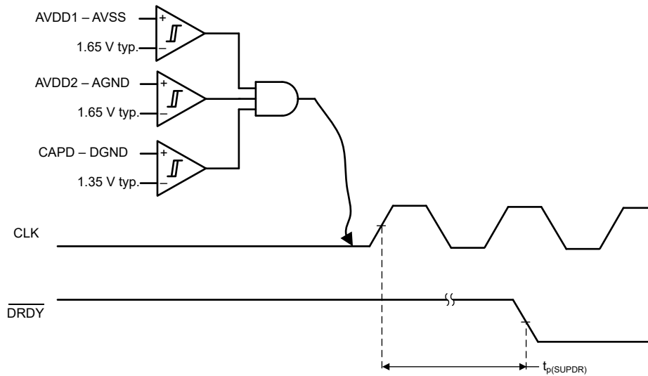
6-8. Power-Up Switching Characteristics
