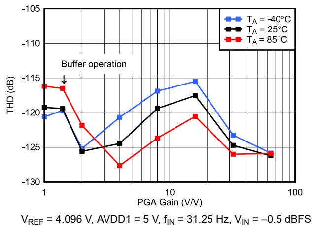
6-50. Mid-Power Mode THD vs PGA Gain
