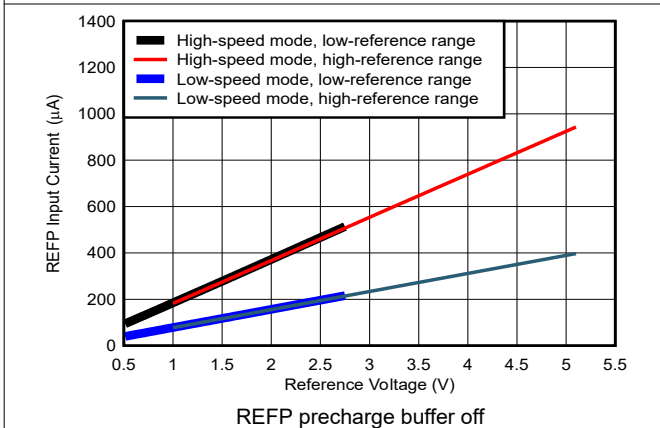
5-83. REFP Input Current vs Reference Voltage
