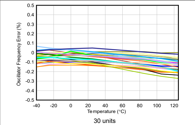
5-80. Oscillator Frequency vs Temperature
