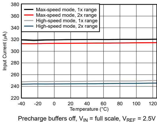
5-45. Input Current vs Temperature
