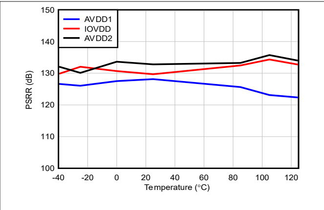
5-86. DC PSRR vs Temperature
