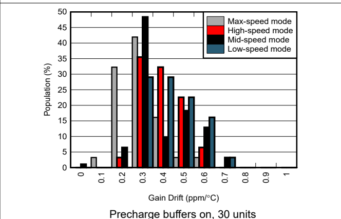
5-54. Gain Drift Distribution
