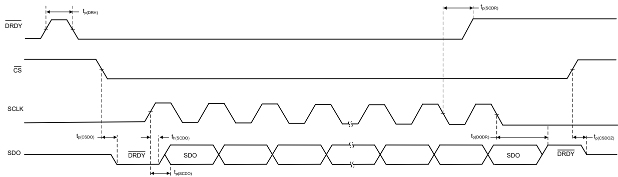
图 5-3. Serial Interface Switching Characteristics
