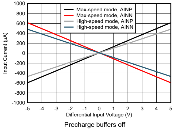
5-43. Input Current vs Differential Voltage
