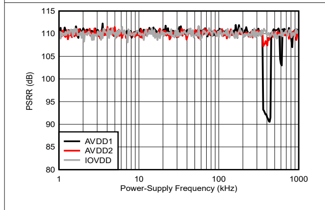
5-87. PSRR vs Power-Supply Frequency
