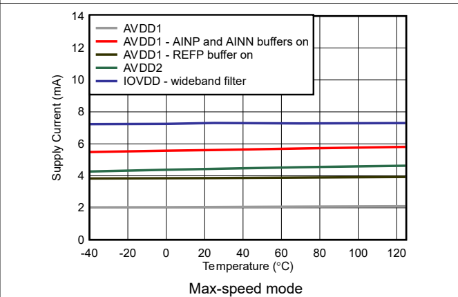
5-88. Power-Supply Current vs Temperature
