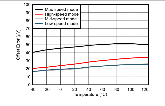
5-50. Offset Error vs Temperature
