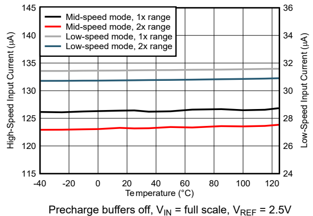
5-46. Input Current vs Temperature
