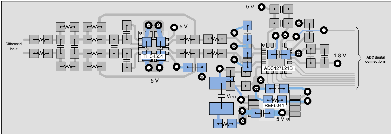
9-14. Layout Example of a Typical Application Circuit
