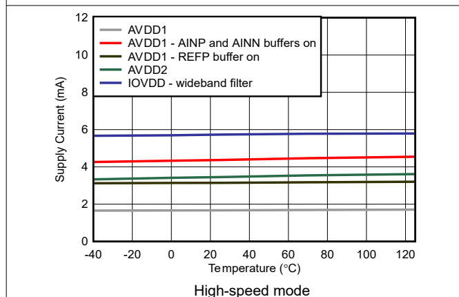
5-89. Power-Supply Current vs Temperature
