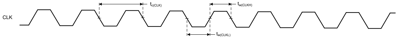
图 5-1. Clock Timing Requirements
