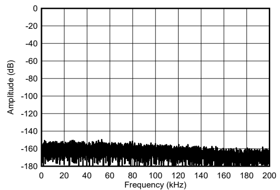
Sinc4 filter
