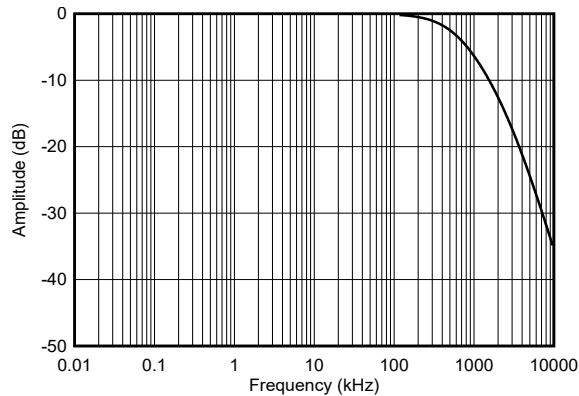
9-7. PGA855 Antialias Filter Response
