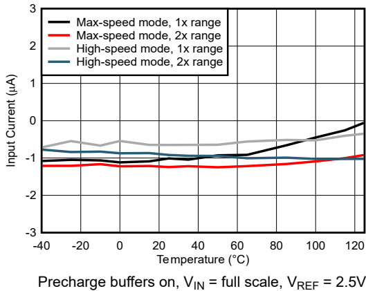
5-47. Input Current vs Temperature
