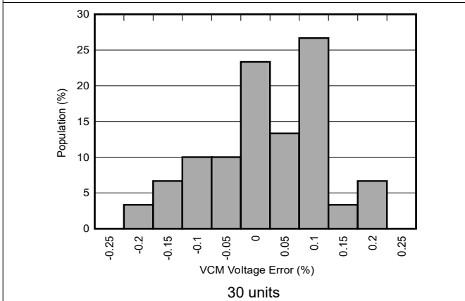
5-81. VCM Voltage Distribution
