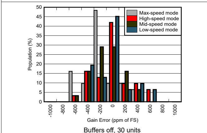
5-53. Gain Error Distribution
