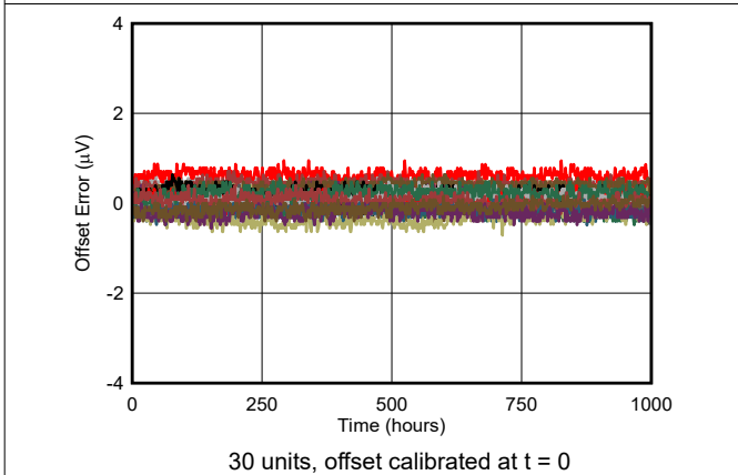
5-51. Long-Term Offset Drift
