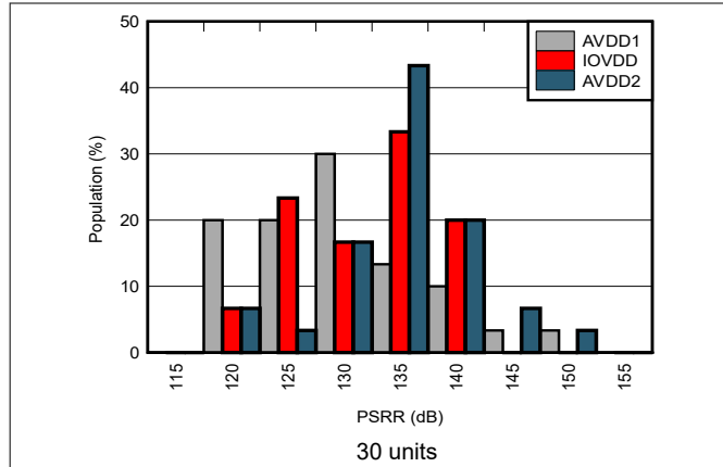
5-85. DC PSRR Distribution
