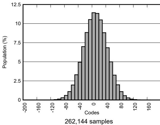
图 5-33. Mid-Speed Mode Code Distributions
