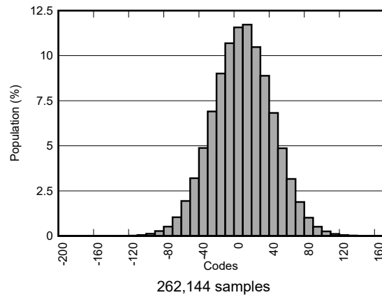
图 5-34. Low-Speed Mode Code Distributions
