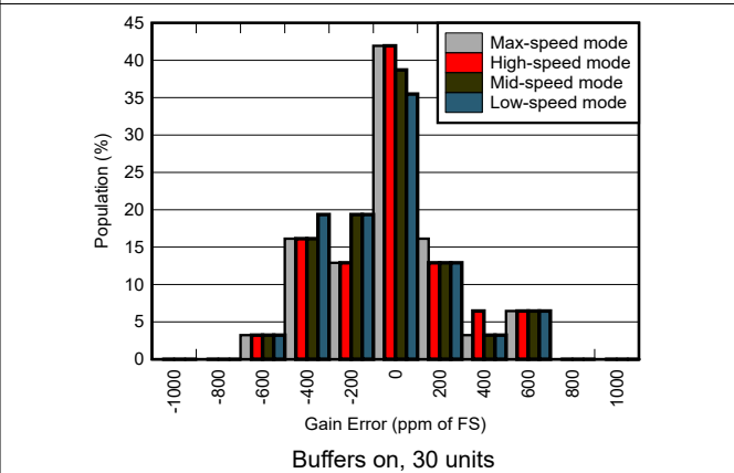
5-52. Gain Error Distribution
