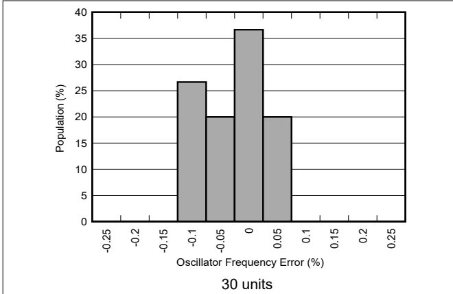
5-79. Oscillator Frequency Distribution
