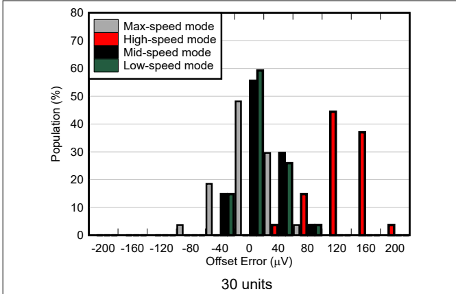
5-49. Offset Error Distribution
