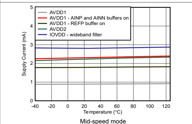
5-90. Power-Supply Current vs Temperature
