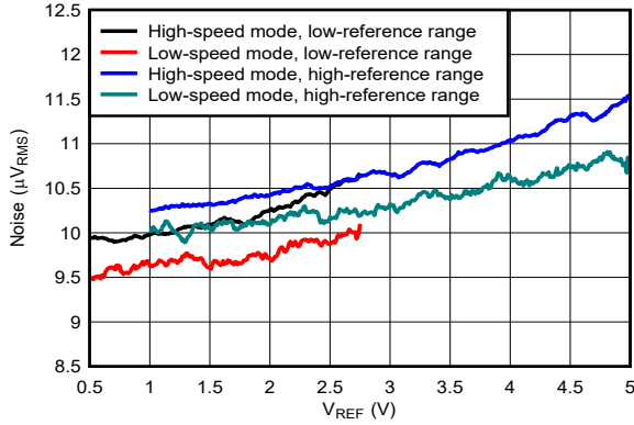
5-37. Noise Performance vs Reference Voltage
