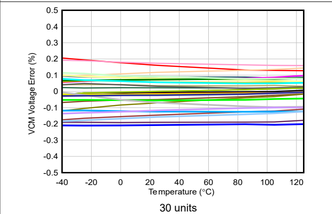
5-82. VCM Voltage vs Temperature
