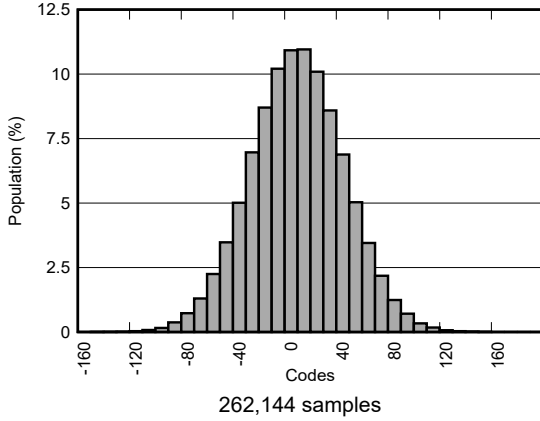
图 5-31. Max-Speed Mode Code Distributions
