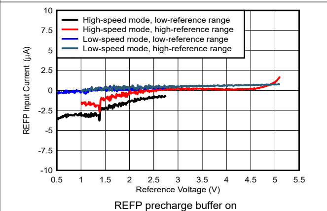
5-84. REFP Input Current vs Reference Voltage
