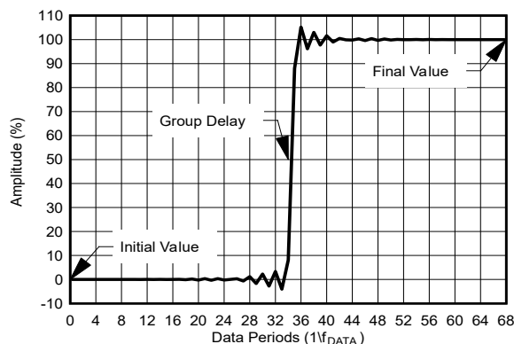
图 7-19. Wideband Filter Step Response
