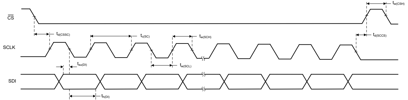
图 5-2. Serial Interface Timing Requirements
