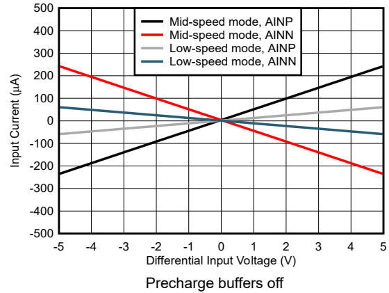
5-44. Input Current vs Differential Voltage
