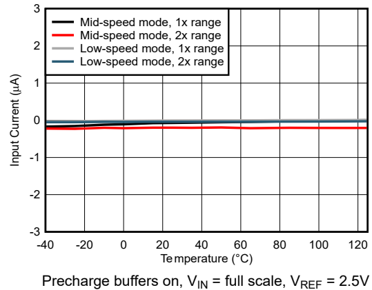
5-48. Input Current vs Temperature
