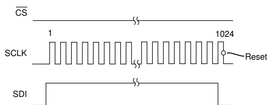
Figure 7-29. Reset Pattern 1 (3-Wire or 4-Wire SPI Mode)
