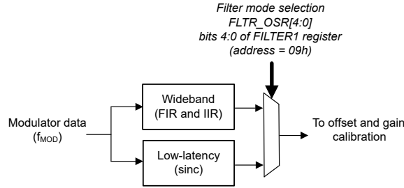
Figure 7-8. Digital Filter Diagram
