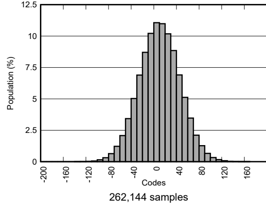
图 5-32. High-Speed Mode Code Distributions
