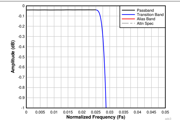
6-29. Decimation by 16 Passband Ripple Response
