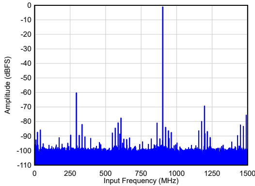
5-5. Single Tone FFT at F_{IN} = 900 MHz
