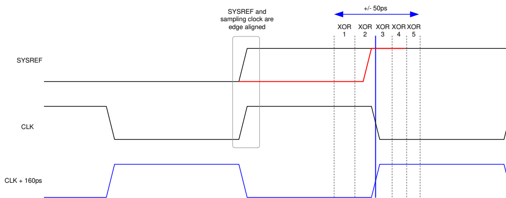
图 6-22. Detection of SYSREF Transition within Capture Window
