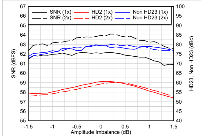
図 6-5. Amplitude Imbalance - 3.0 GSPS
