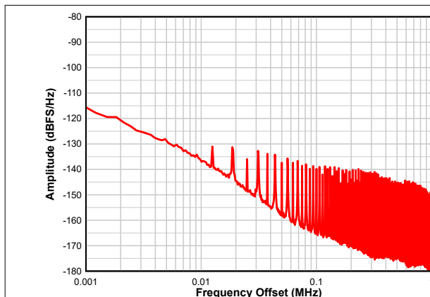
Figure 6-8. Dither Close-Up
