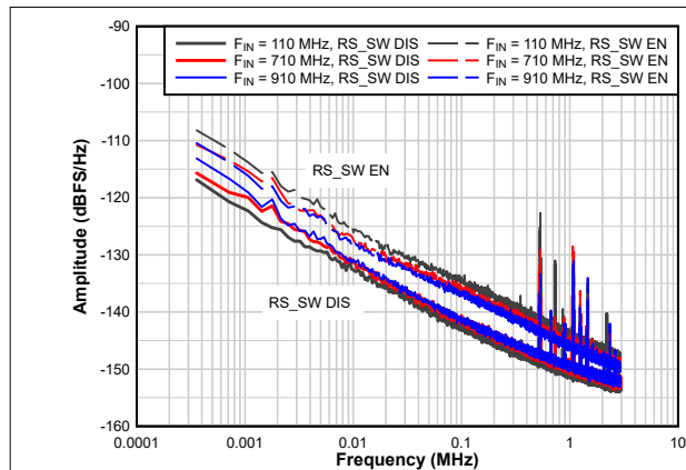
図 6-10. Amplitude Noise vs Input Frequency
