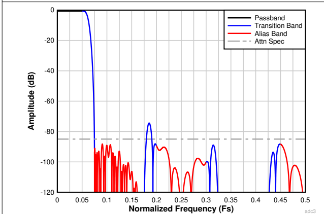
6-26. Complex Decimation by 8 Filter Response
