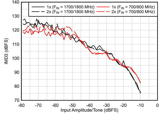
5-30. IMD3 Performance vs A_{IN}
