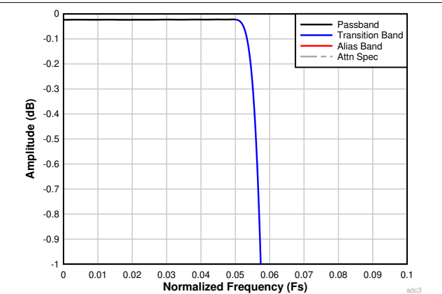
6-27. Decimation by 8 Passband Ripple Response
