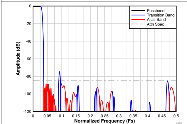
6-28. Complex Decimation by 16 Filter Response
