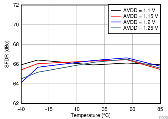
f_{IN} = 1.78 GHz, A_{IN} = -2 dBFS
