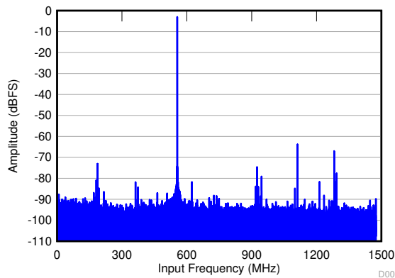
Fig 6-11. FFT for 2600-MHz Input Signal
