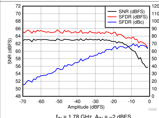
6-58. Performance vs. Amplitude
