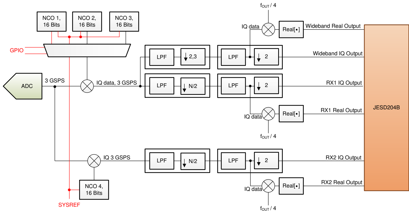
8-14. DDC Chains Overview (One ADC Channel Shown)
