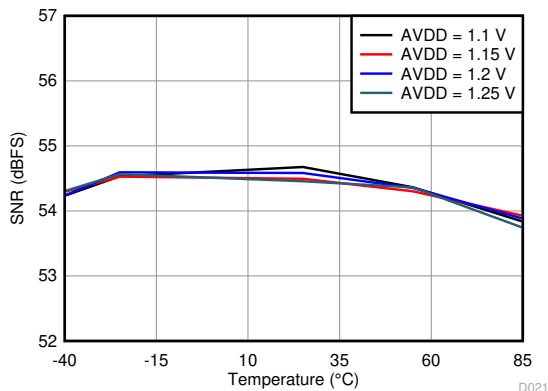
f_{IN} = 3.5 GHz, A_{IN} = -3 dBFS with 2-dB digital gain
