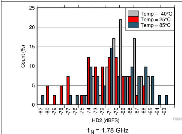
6-57. HD2 Histogram at AVDD19 = 2.0 V
