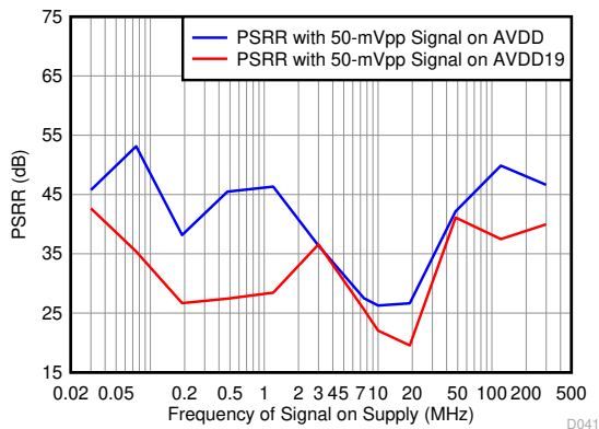
6-65. Power-Supply Rejection Ratio vs. Tone Frequency
