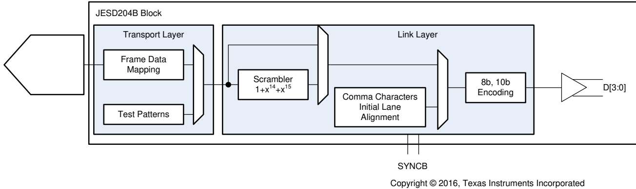
8-54. JESD Digital Block Implementation
