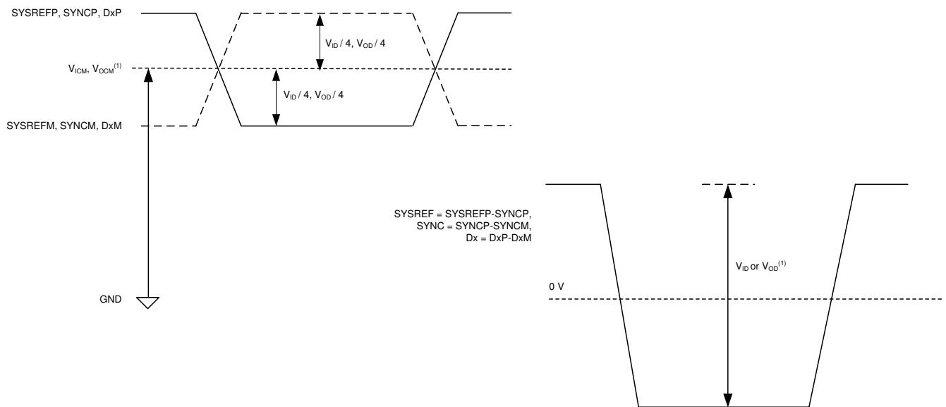
6-1. Logic Levels for Digital Inputs and Outputs
