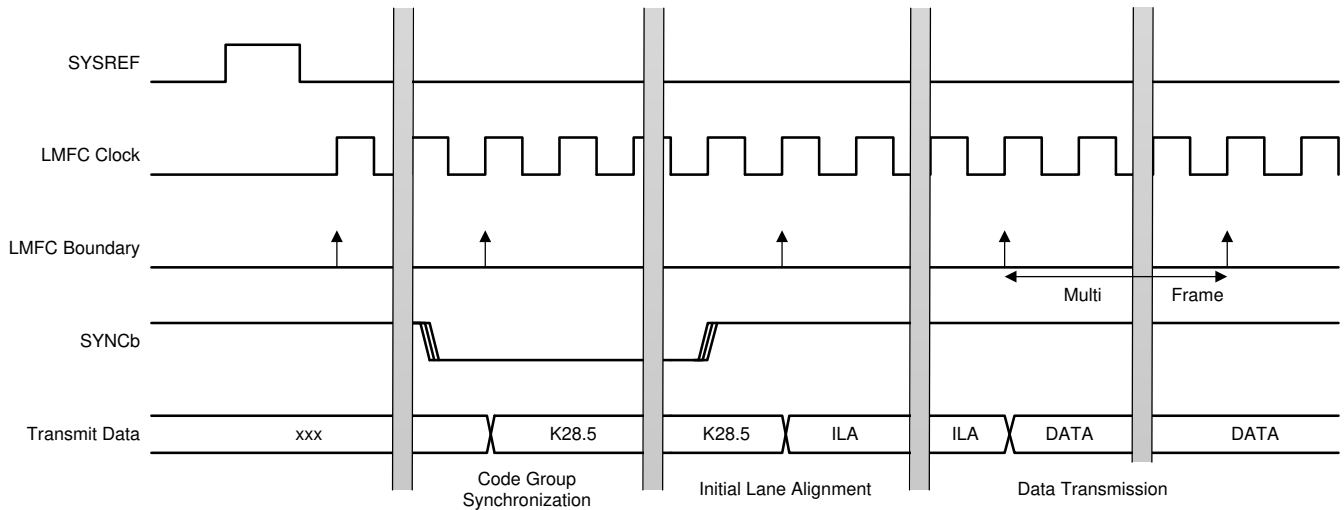
8-55. JESD Internal Timing Information
