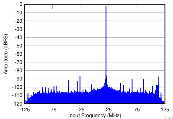
FIG 6-71. FFT in 9x Decimation (Complex Output)
