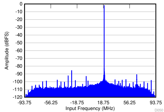
FIG 6-72. FFT in 10x Decimation (Complex Output)
