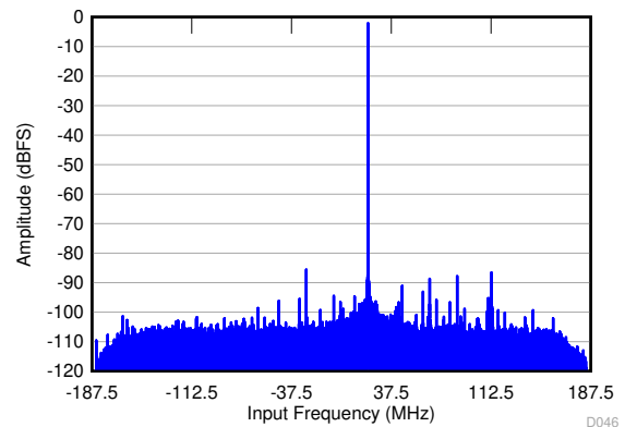
f_{IN} = 1.78 GHz, A_{IN} = -2 dBFS, f_S = 2949.12 MSPS, SNR = 62.6 dBFS, SFDR (includes IL) = 86 dBc
