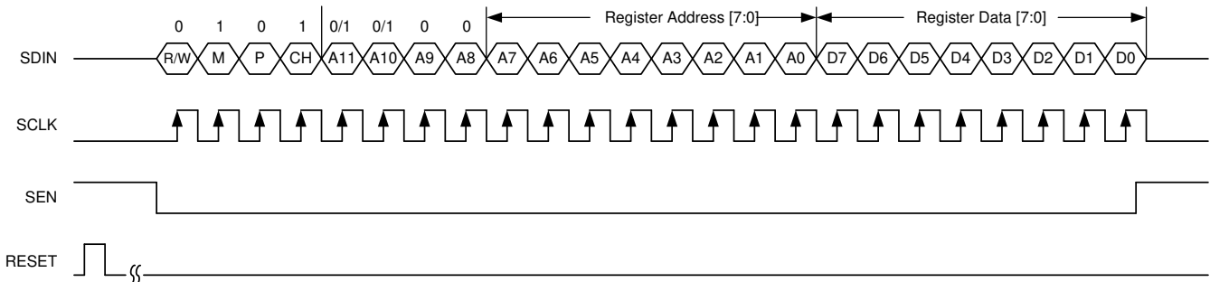
8-63. SPI Write Timing Diagram for the Decimation and Power Detector Pages
