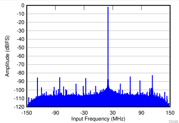
FIG 6-72. FFT in 10x Decimation (Complex Output)
