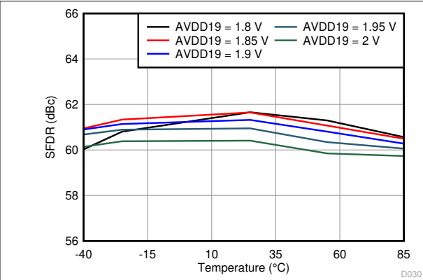
f_{IN} = 3.5 \text{ GHz} , A_{IN} = -3 \text{ dBFS} with 2-dB digital gain
