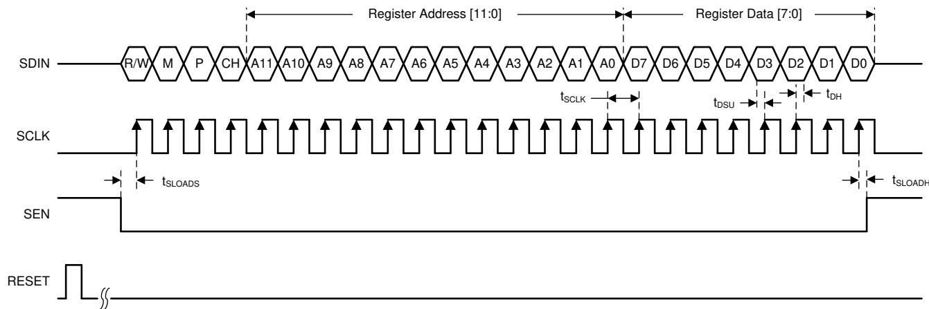
图 8-56. SPI Timing Diagram
