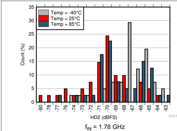
6-55. HD2 Histogram at AVDD19 = 1.8 V
