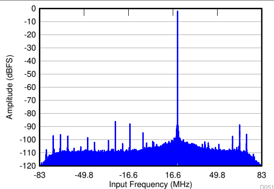
FIG 6-73. FFT in 12x Decimation (Complex Output)
