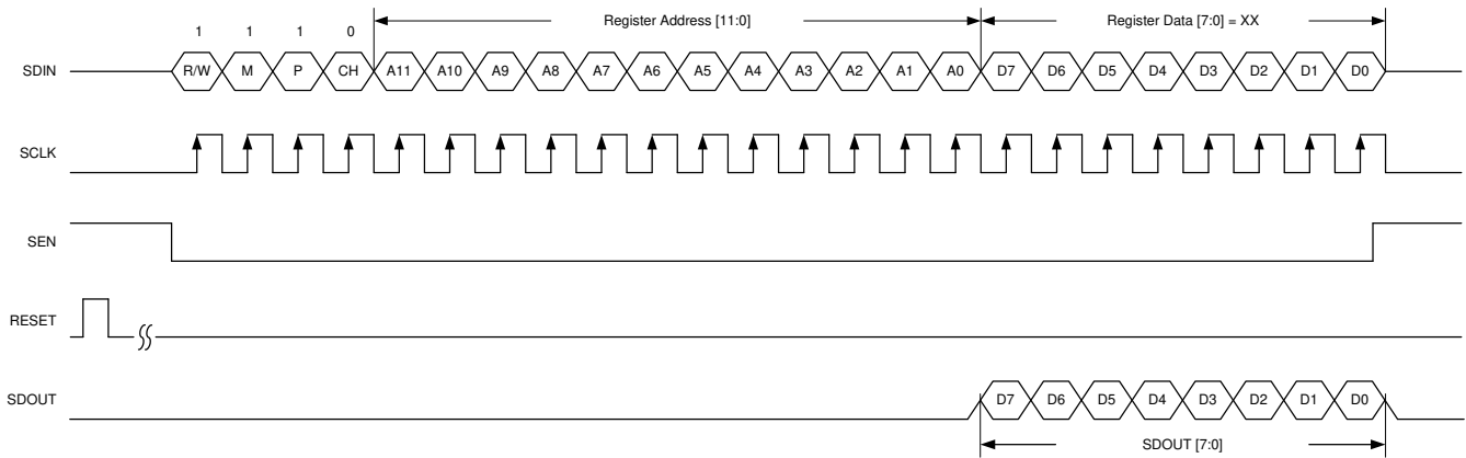
8-62. SPI Read Timing Diagram for the Digital Bank
