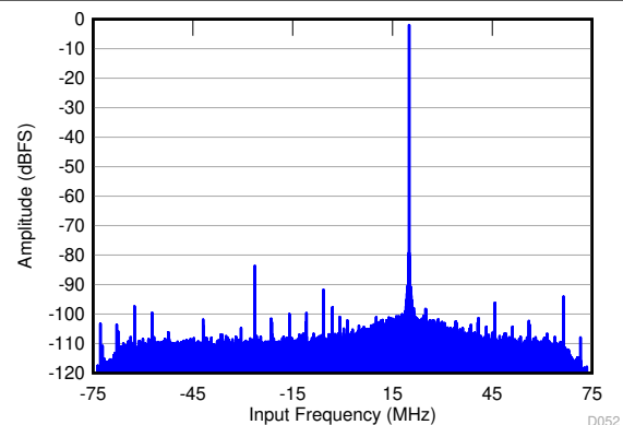
FIG 6-74. FFT in 16x Decimation (Complex Output)
