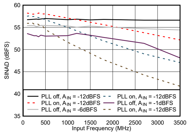
5-26. SINAD vs Input Frequency
