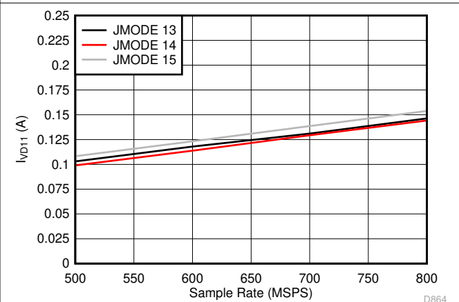
5-110. Single Channel, I_{VD11} vs F_S for JMODES 13 - 15
