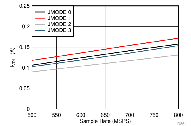
5-107. Single Channel, I_{VD11} vs F_S for JMODES 0 - 3
