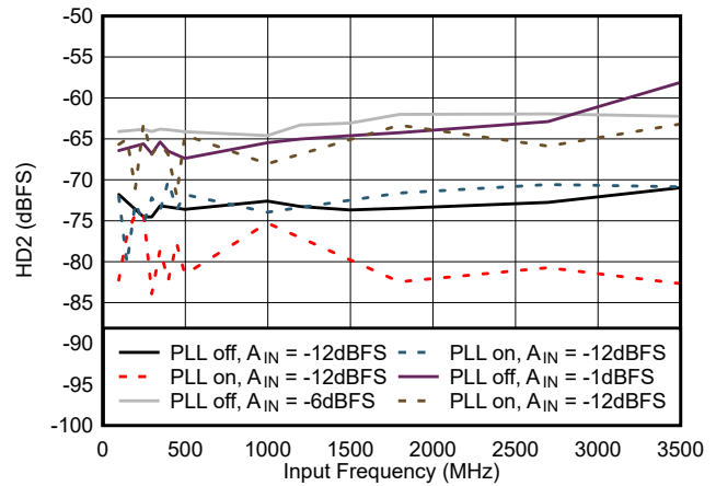
5-24. HD2 vs Input Frequency
