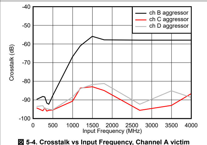
図 5-4. Crosstalk vs Input Frequency, Channel A victim
