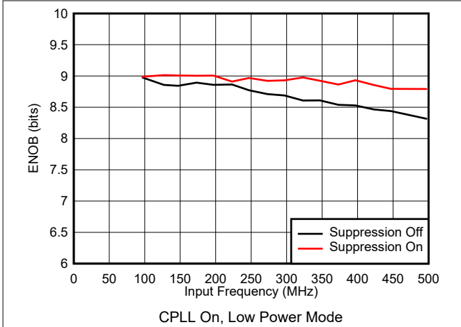
Figure 5-63. ENOB vs Input Frequency
