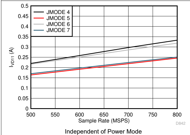
图 5-81. Quad Channel, I_{VD11} vs F_S for JMODES 4 - 7
