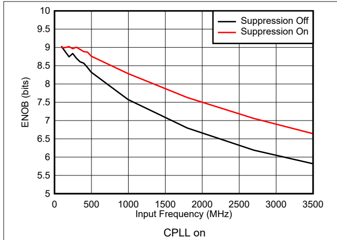
Figure 5-37. ENOB vs Input Frequency and Suppression
