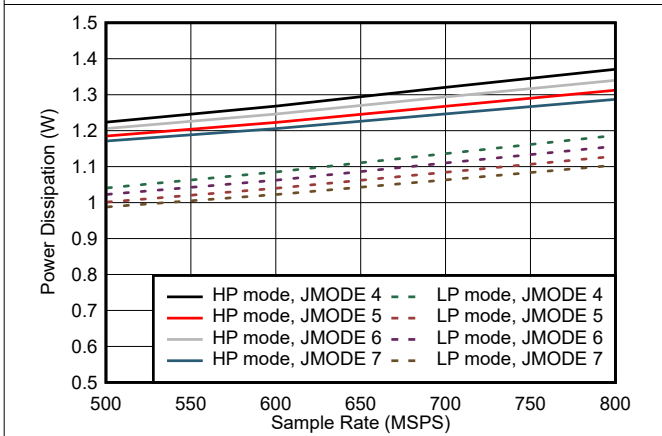
Figure 5-89. Dual Channel, Power Dissipation vs F_S for JMODES 4 - 7
