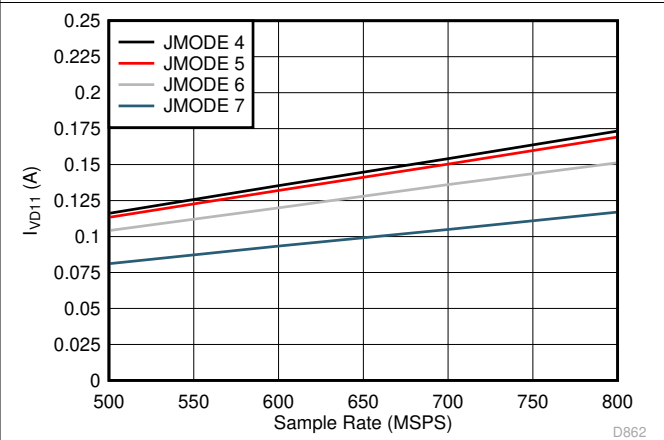
5-108. Single Channel, I_{VD11} vs F_S for JMODES 4 - 7
