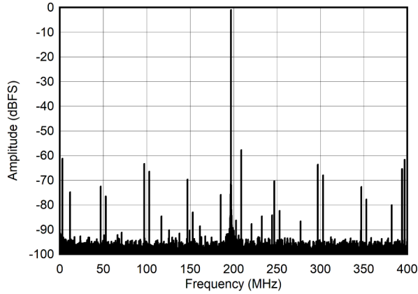
5-21. Single Tone FFT at 997 MHz and -1dBFS
