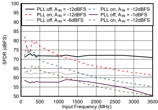
5-23. SFDR vs Input Frequency
