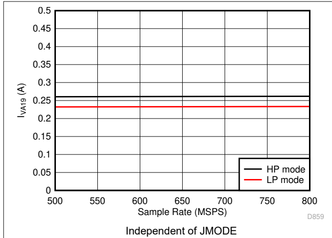
5-105. Single Channel, I_{VA19} vs F_S
