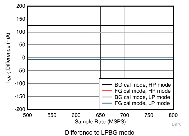
5-112. Single Channel, I_{VA19} vs F_S over Modes
