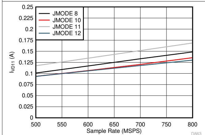
5-109. Single Channel, I_{VD11} vs F_S for JMODES 8 - 12
