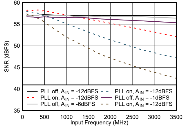
5-22. SNR vs Input Frequency
