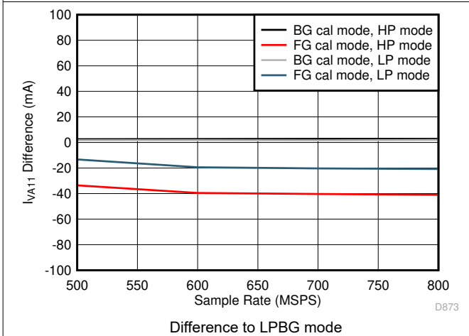
5-113. Single Channel, I_{VA11} vs F_S over Modes
