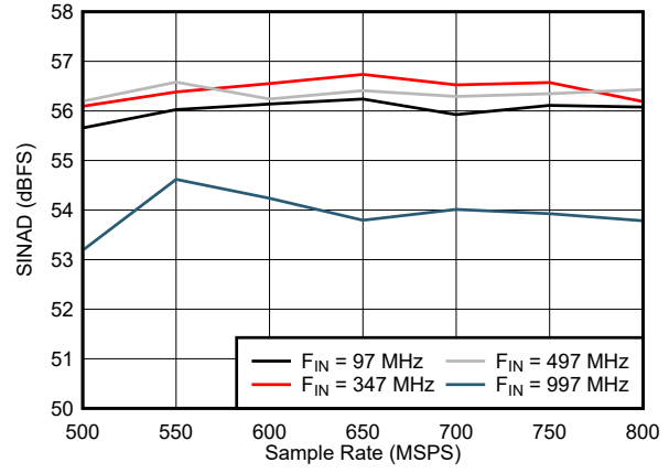
Figure 5-56. SINAD vs Sample Rate in Low Power Mode
