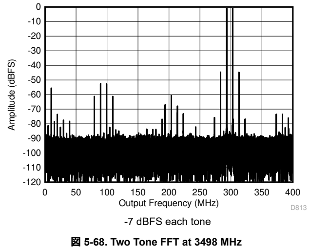
Figure 5-68. Two Tone FFT at 3498 MHz
