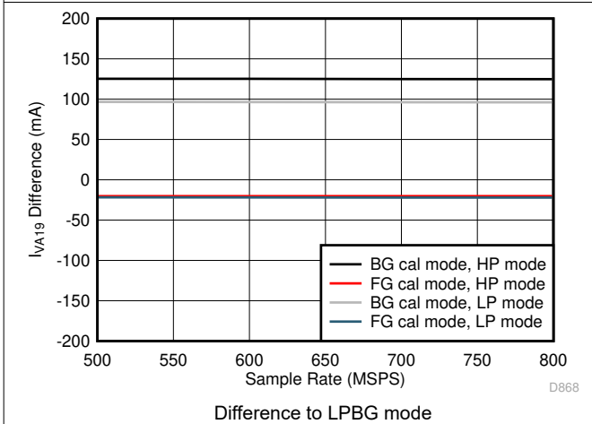
5-85. Quad Channel, I_{VA19} vs F_S over Modes
