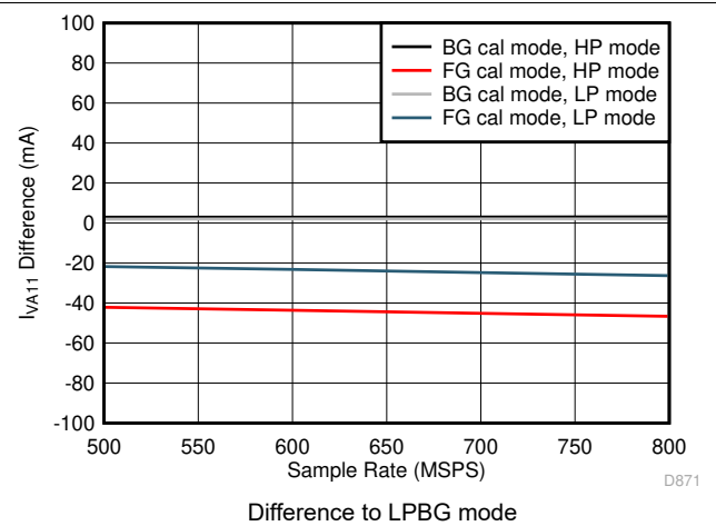
5-86. Quad Channel, I_{VA11} vs F_S over Modes
