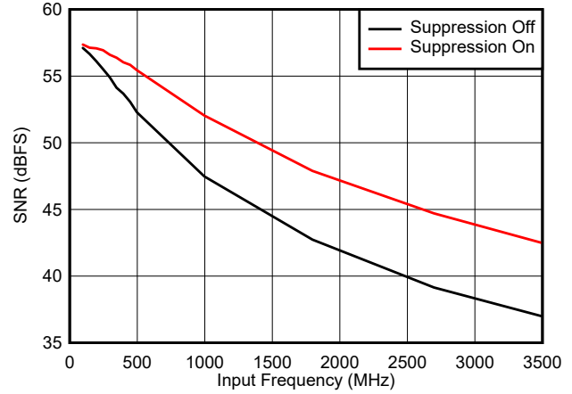
图 5-34. SNR vs Input Frequency and Suppression
