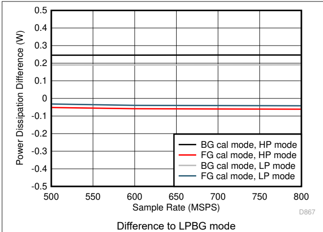
5-111. Single Channel, Power Dissipation vs F_S over Modes
