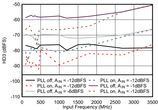
5-25. HD3 vs Input Frequency
