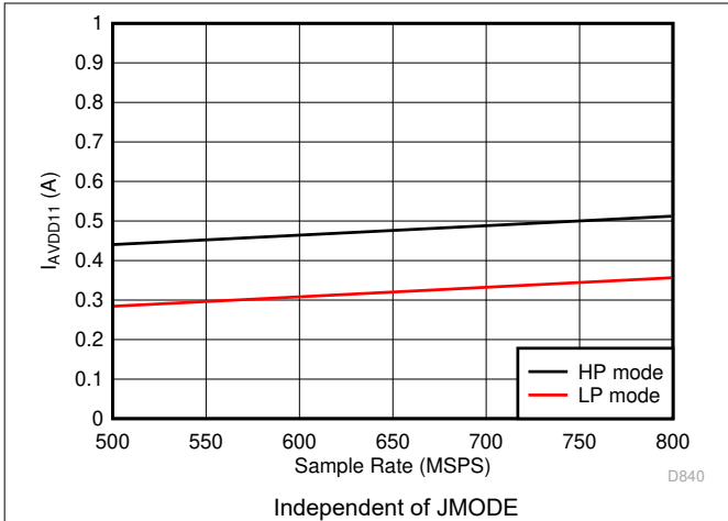
图 5-79. Quad Channel, I_{VA11} vs F_S
