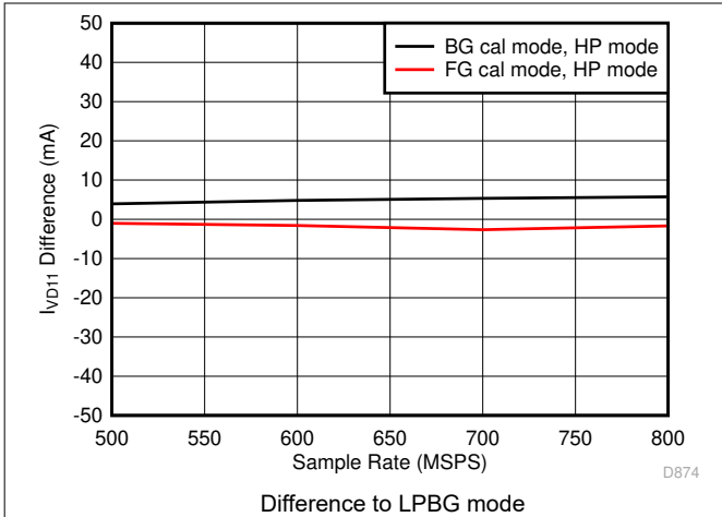
Figure 5-87. Quad Channel, I_{VD11} vs F_S over Modes
