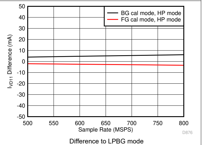
5-114. Single Channel, I_{VD11} vs F_S over Modes
