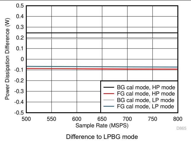
5-84. Quad Channel, Power Dissipation vs F_S over Modes
