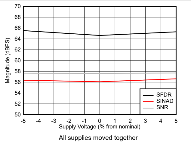
Figure 5-38. SNR, SFDR and SINAD vs Supply Voltage
