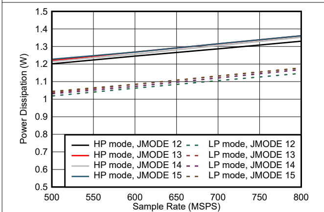
Figure 5-91. Dual Channel, Power Dissipation vs F_S for JMODES 12 - 15
