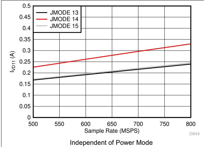
5-83. Quad Channel, I_{VD11} vs F_S for JMODES 13-15
