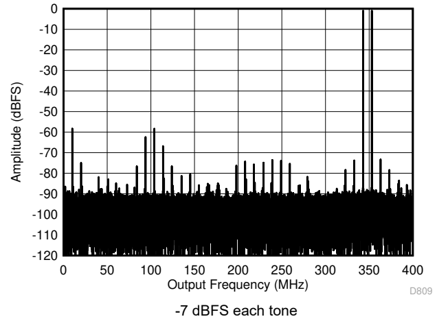
Figure 5-66. Two Tone FFT at 347 MHz
