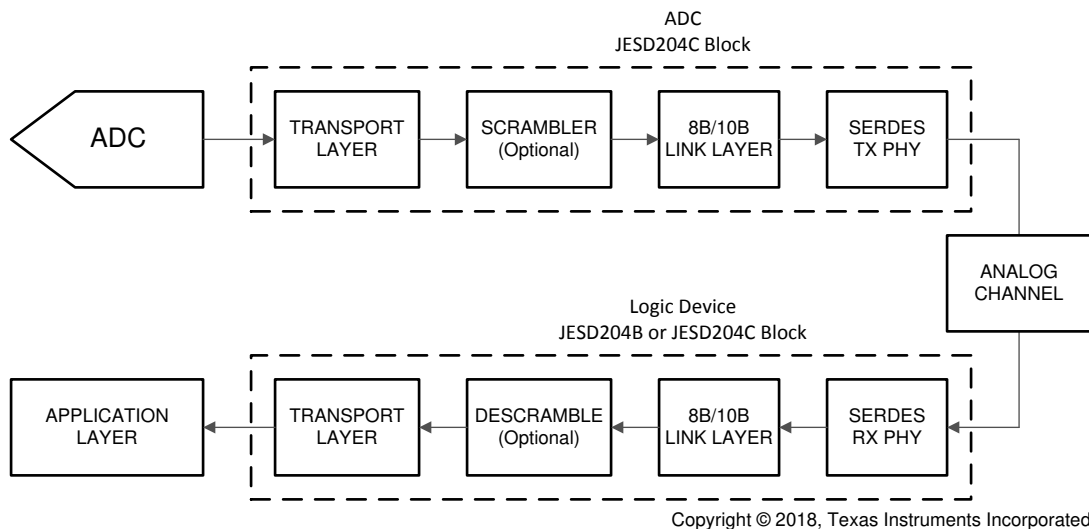
6-5. Simplified 8B/10B Encoded JESD204C Interface Diagram
