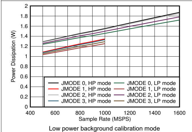
5-89. Dual Channel, Power Dissipation vs F_S and JMODE 0 - 3
