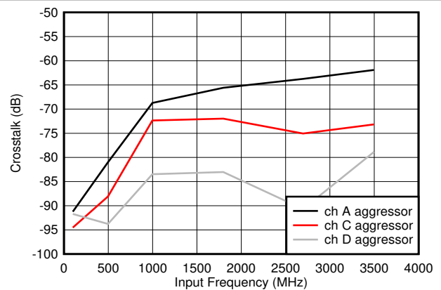
图 5-78. Crosstalk to Channel B vs F_{IN}
