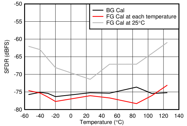
5-68. Worst Spur vs Temperature
