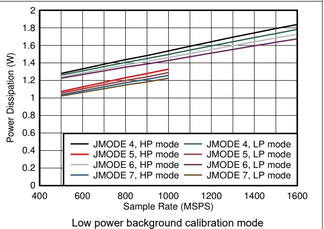
5-90. Dual Channel, Power Dissipation vs F_S and JMODE 4 - 7
