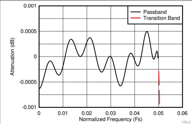
6-14. Decimate-by-8 Composite Zoomed Pass-Band Response
