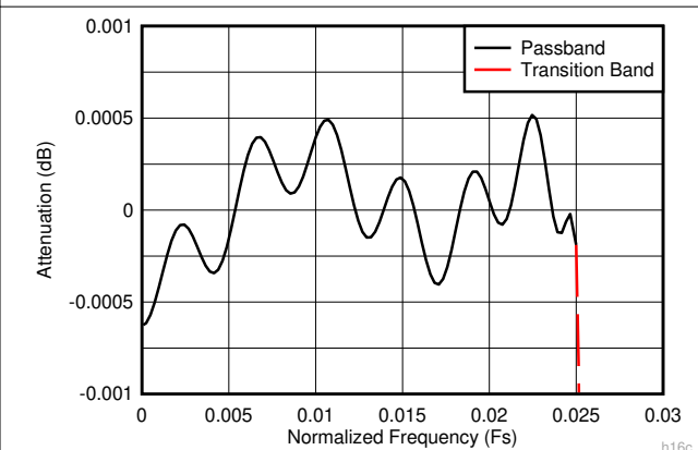
6-16. Decimate-by-16 Composite Zoomed Pass-Band Response
