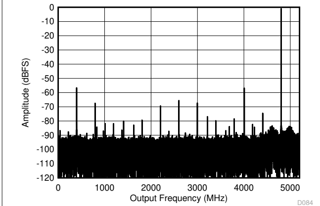
5-9. DES Mode: Single Tone FFT at 5597 MHz
