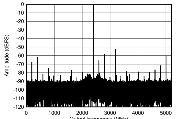
5-10. DES Mode: Single Tone FFT at 7997 MHz
