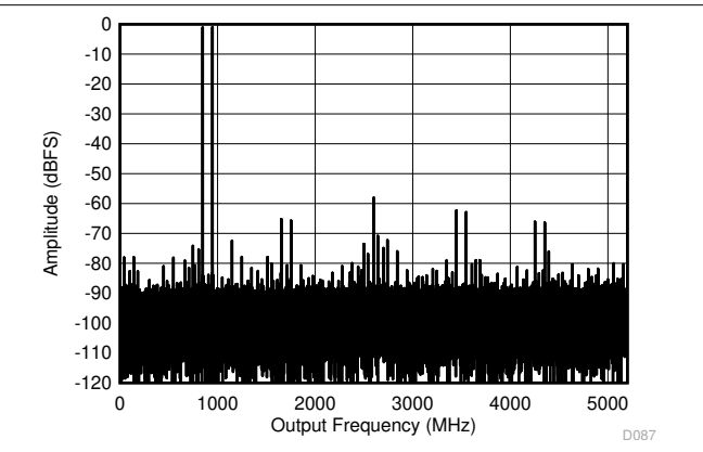
5-12. DES Mode: Two Tone FFT at 897 MHz
