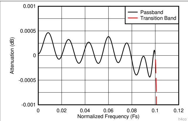
6-12. Decimate-by-4 Composite Zoomed Pass-Band Response
