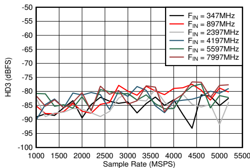
5-55. Dual Channel Mode: HD3 vs Sample Rate and Input Frequency A_{IN} = -1\text{ dBFS}
