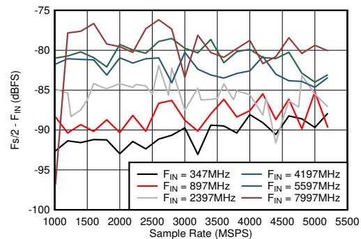
5-58. Dual Channel Mode: F_s/2 - F_{IN} vs Sample Rate and Input Frequency
