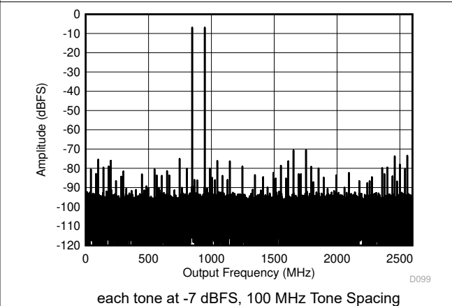
5-24. Dual Channel Mode: Two Tone FFT at 897 MHz
