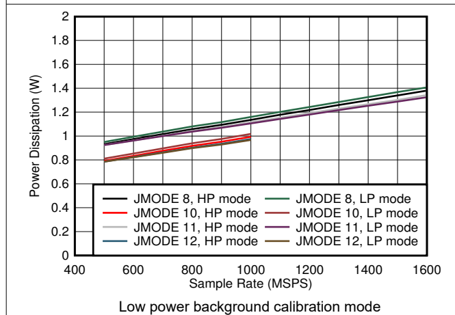
6-101. Single Channel, Power Dissipation vs F_S and JMODE 8 - 12
