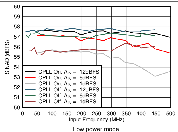
Figure 6-56. SINAD vs A_{IN} and C-PLL
