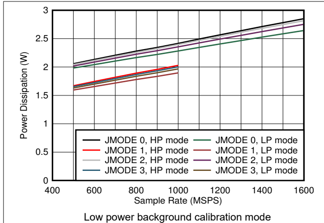
6-79. Quad Channel, Power Dissipation vs F_S and JMODES 0 - 3
