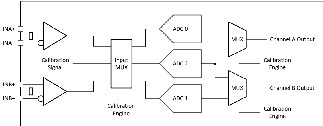
7-16. DualChannel Calibration System Block Diagram
