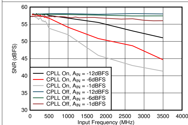
Figure 6-49. SNR vs A_{IN} and C-PLL
