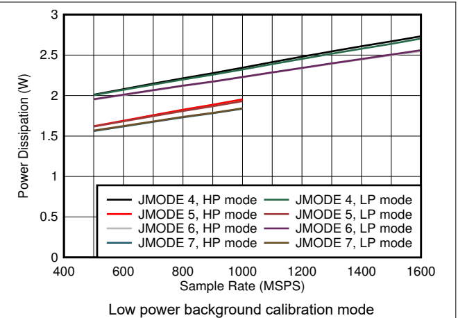
6-80. Quad Channel, Power Dissipation vs F_S and JMODE 4 - 7
