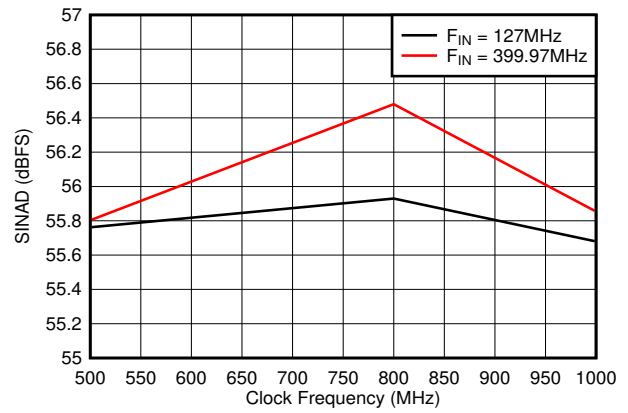
Figure 6-30. SINAD vs Sample Rate
