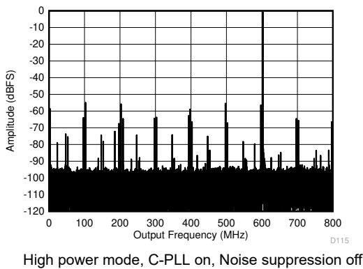
6-9. Single Tone FFT at 997 MHz and -1 dBFS
