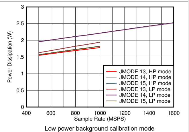
6-82. Quad Channel, Power Dissipation vs F_S and JMODE 13 - 15
