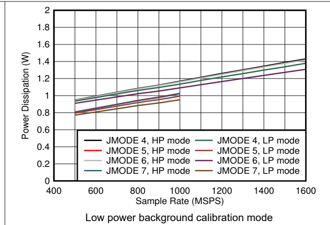
6-100. Single Channel, Power Dissipation vs F_S and JMODE 4 - 7
