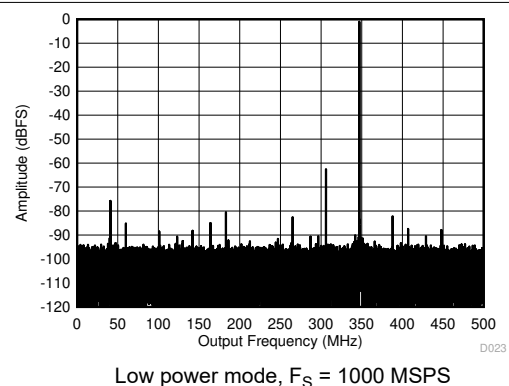
6-12. Single Tone FFT at 347 MHz and -1 dBFS
