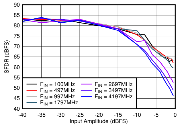
Figure 6-32. SFDR vs A_{IN}
