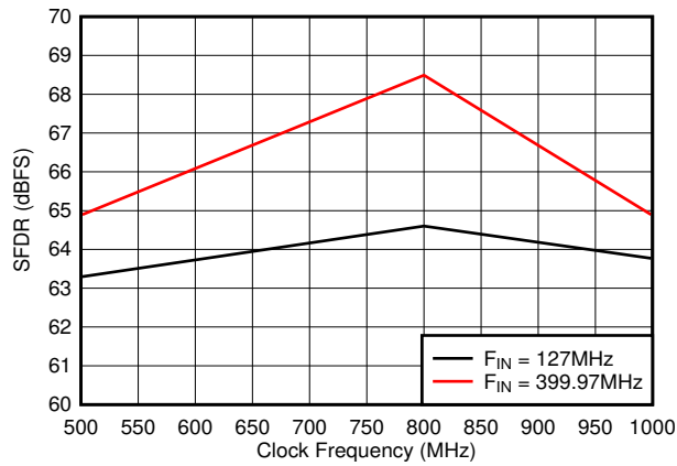
Figure 6-29. SFDR vs Sample Rate
