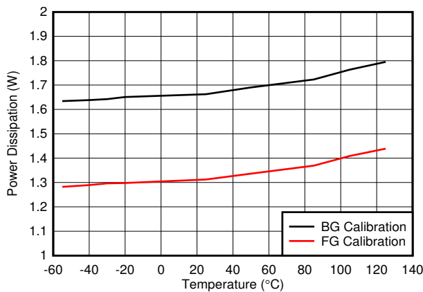
6-121. Quad Channel, Power Dissipation vs Temperature
