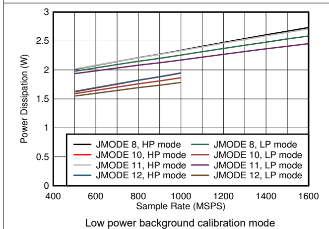
6-81. Quad Channel, Power Dissipation vs F_S and JMODE 8 - 12
