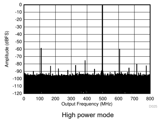
6-10. Single Tone FFT at 1797 MHz and -1 dBFS
