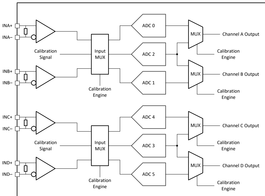
7-15. Quad Channel Calibration System Block Diagram
