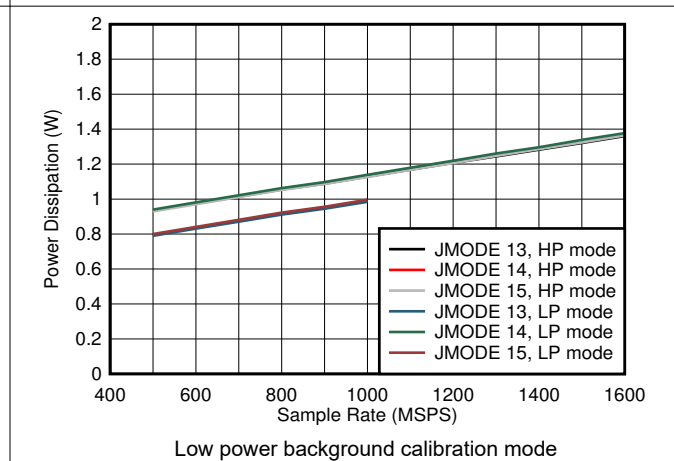
6-102. Single Channel, Power Dissipation vs F_S and JMODE 13 - 15
