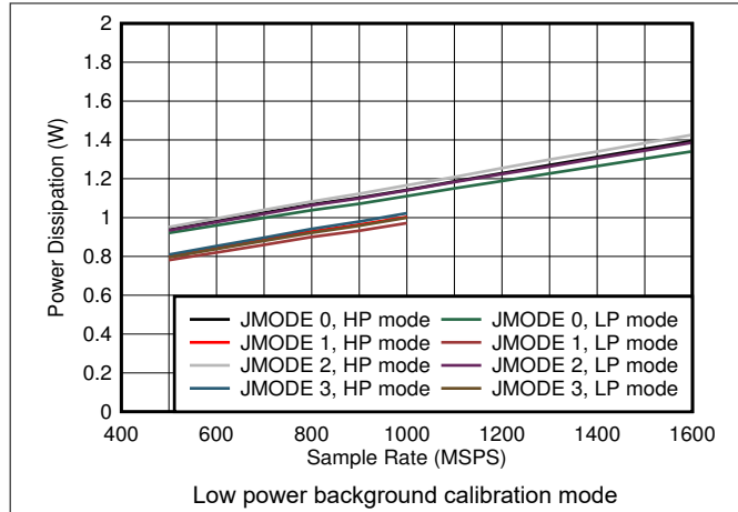
6-99. Single Channel, Power Dissipation vs F_S and JMODE 0 - 3
