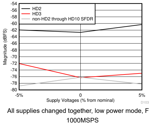
Figure 6-63. HD2, HD3 and Worst non-HD Spur vs Supply Voltage
