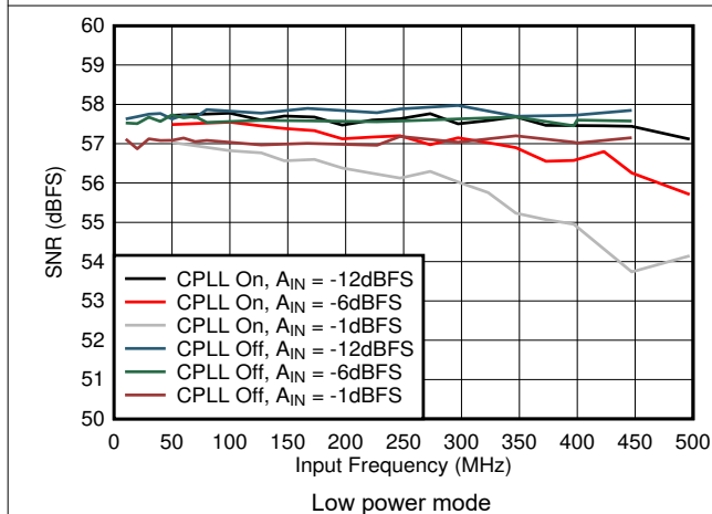
Figure 6-55. SNR vs A_{IN} and C-PLL
