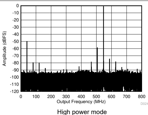
6-11. Single Tone FFT at 3797 MHz and -1 dBFS
