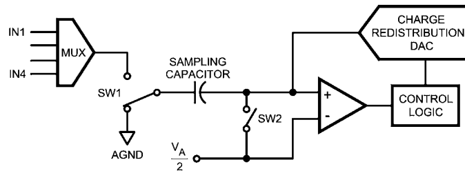
FIGURE 2. ADC124S051 in Hold Mode
