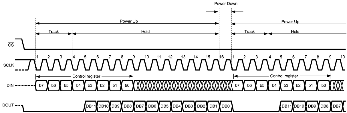
ADC124S051 Operational Timing Diagram
