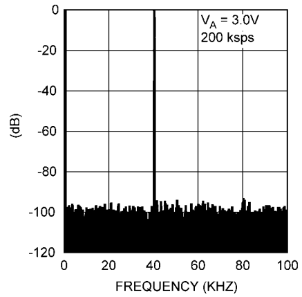
Spectral Response - 3V, 200 kSPS
