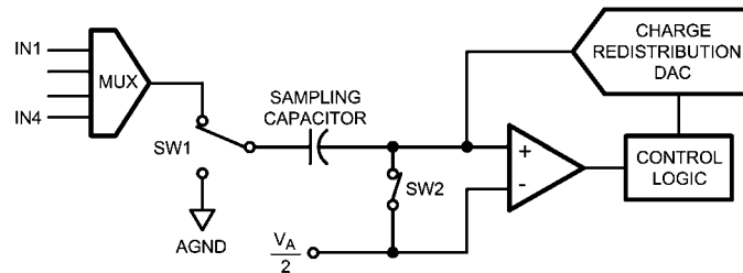
FIGURE 1. ADC124S051 in Track Mode
