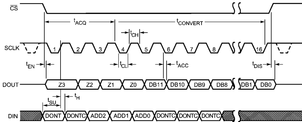
ADC124S051 Serial Timing Diagram
