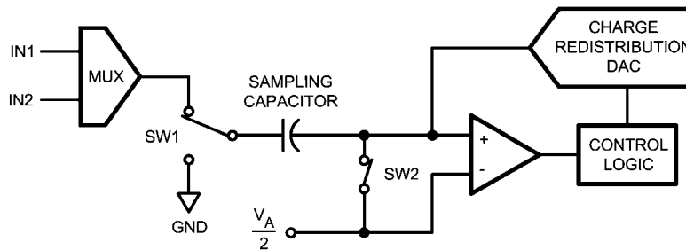
FIGURE 1. ADC122S051 in Track Mode
