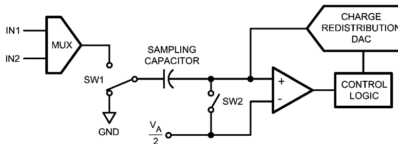
FIGURE 2. ADC122S051 in Hold Mode
