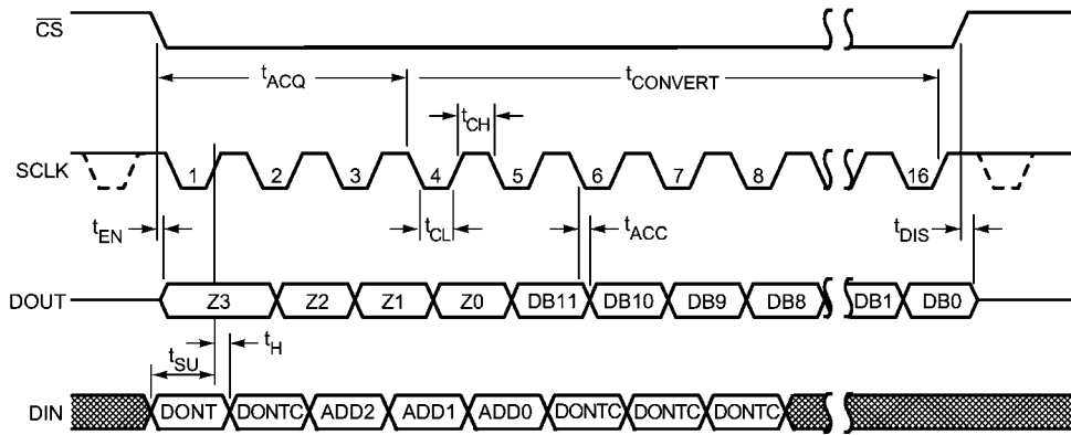
ADC122S051 Serial Timing Diagram
