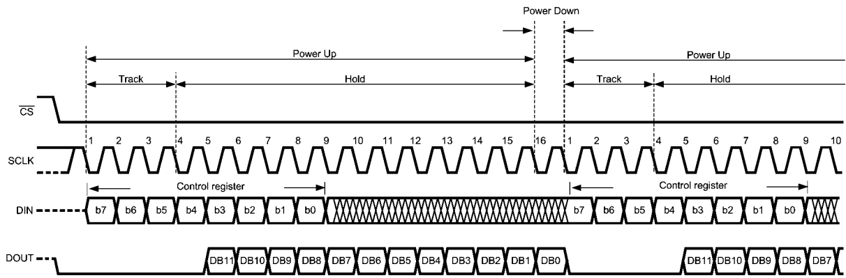
ADC122S051 Operational Timing Diagram
