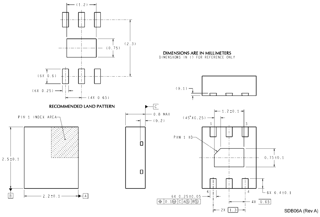
6-Lead LLP Order Number ADC121S101CISD or ADC121S101CISDX NS Package Number SDB06A 単位は millimeters
