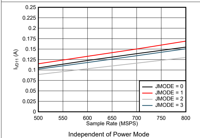
Figure 5-97. Single Channel, I_{VD11} vs F_S for JMODES 0 - 3
