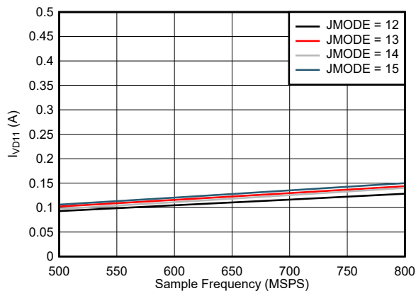
5-100. Single Channel, I_{VD11} vs F_S for JMODES 12 - 15
