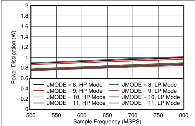
Figure 5-93. Single Channel, Power Dissipation vs F_S for JMODES 8 - 11
