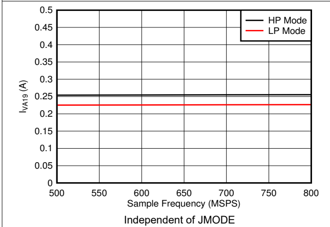
Figure 5-95. Single Channel, I_{VA19} vs F_S
