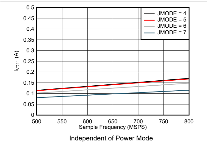
Figure 5-98. Single Channel, I_{VD11} vs F_S for JMODES 4 - 7
