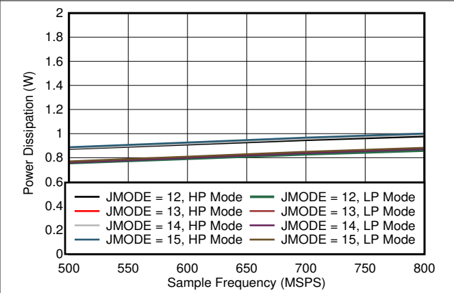
Figure 5-94. Single Channel, Power Dissipation vs F_S for JMODES 12 - 15
