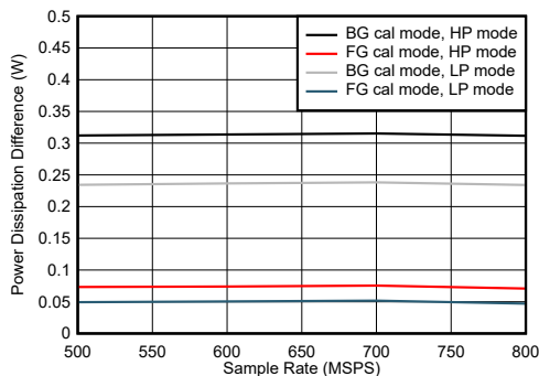
5-101. Quad Channel, Power Dissipation Change with Calibration Mode
