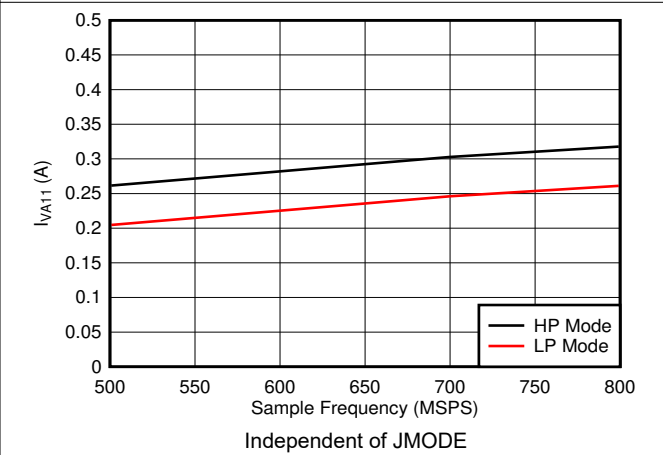
Figure 5-96. Single Channel, I_{VA11} vs F_S
