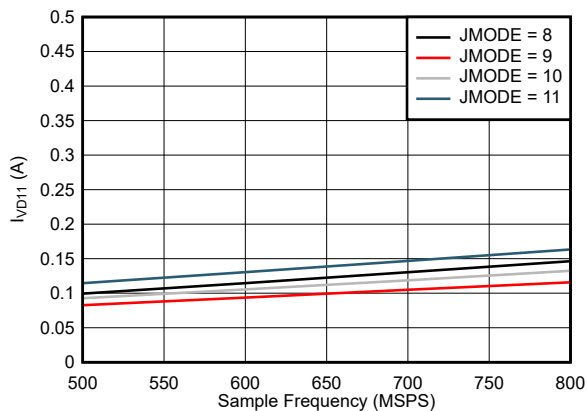
5-99. Single Channel, I_{VD11} vs F_S for JMODES 8 - 11
