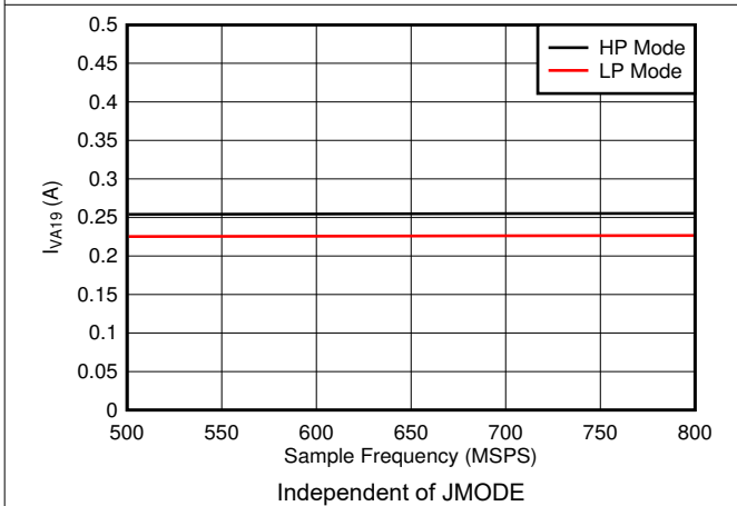
图 5-95. Single Channel, I_{VA19} vs F_S
