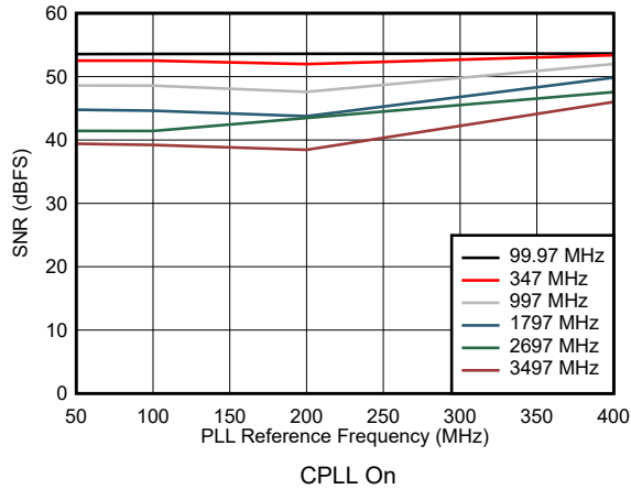
5-63. SNR vs Reference Clock Frequency
