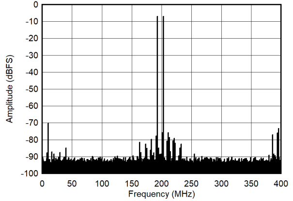
Low Power Mode, -7 dBFS each tone 图 5-58. Dual Tone FFT at 998 MHz (LP Mode)
