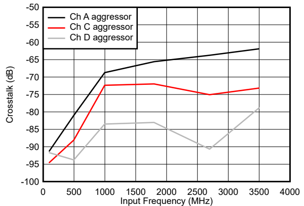
Channel B victim 图 5-62. Crosstalk vs Input Frequency
