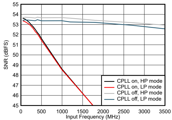
5-66. SNR vs Input Frequency and CPLL and Power Mode
