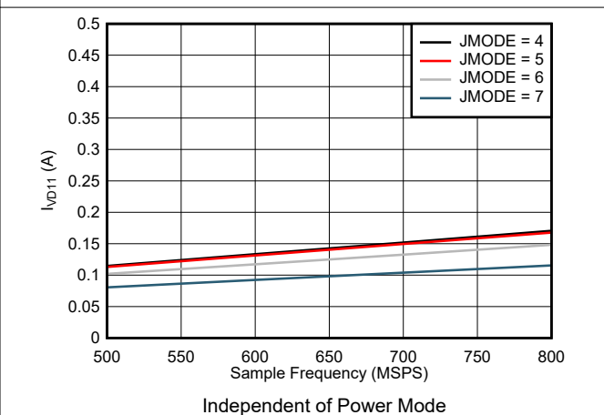
图 5-98. Single Channel, I_{VD11} vs F_S for JMODES 4 - 7
