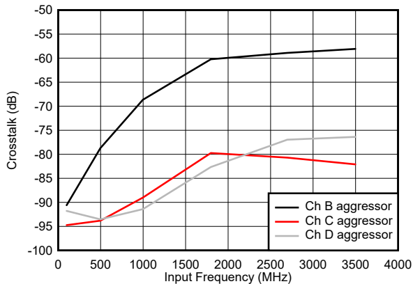
Channel A victim 图 5-61. Crosstalk vs Input Frequency
