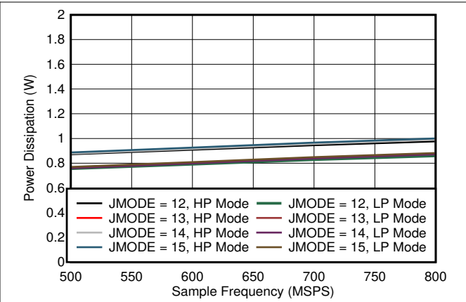
图 5-94. Single Channel, Power Dissipation vs F_S for JMODES 12 - 15
