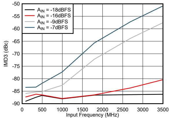
Low Power Mode, 10 MHz Tone Spacing 图 5-60. IMD3 vs Input Frequency (LP Mode)
