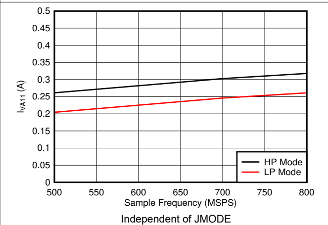
图 5-96. Single Channel, I_{VA11} vs F_S
