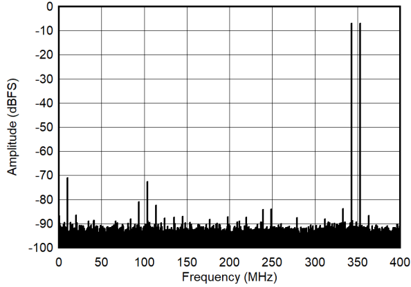
Low Power Mode, -7 dBFS each tone 图 5-57. Dual Tone FFT at 348 MHz (LP Mode)
