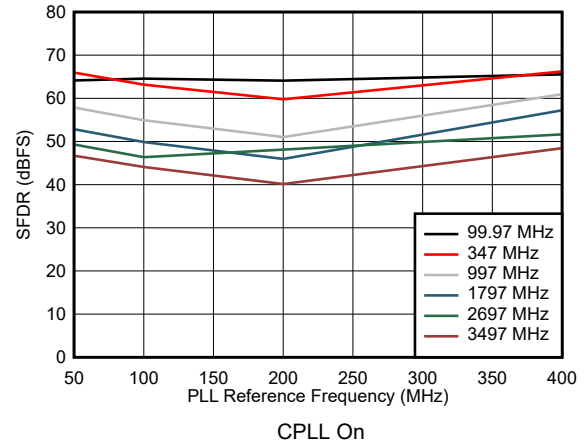
5-64. SFDR vs Reference Clock Frequency
