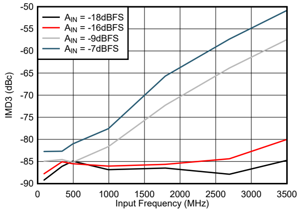
10 MHz Tone Spacing 图 5-59. IMD3 vs Input Frequency
