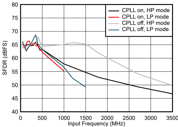
5-65. SFDR vs Input Frequency and CPLL and Power Mode
