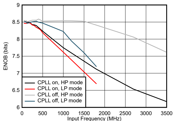
5-68. ENOB vs Input Frequency and CPLL and Power Mode
