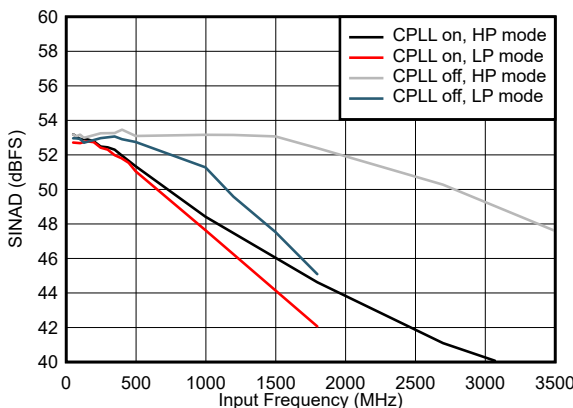
5-67. SINAD vs Input Frequency and CPLL and Power Mode
