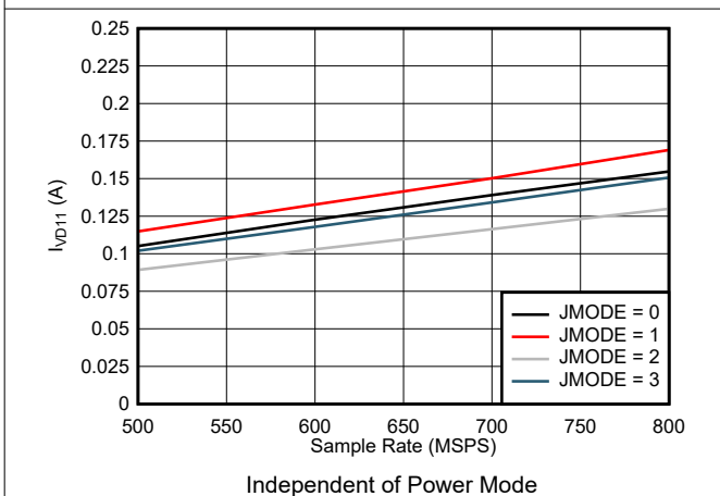
图 5-97. Single Channel, I_{VD11} vs F_S for JMODES 0 - 3
