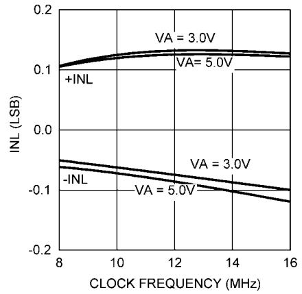
INL vs. Clock Frequency
