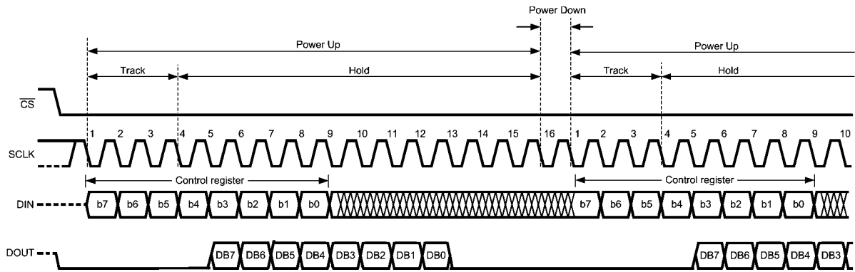
ADC084S101 Operational Timing Diagram
