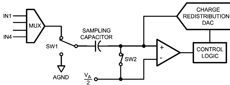
FIGURE 1. ADC084S051 in Track Mode
