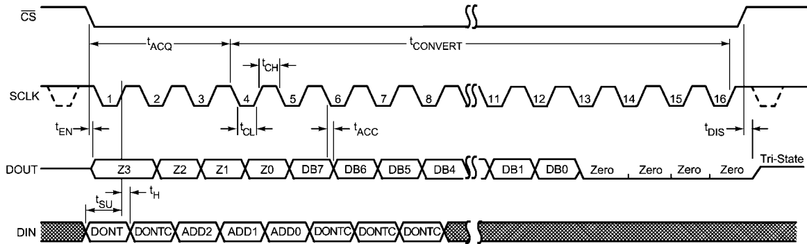
ADC084S051 Serial Timing Diagram
