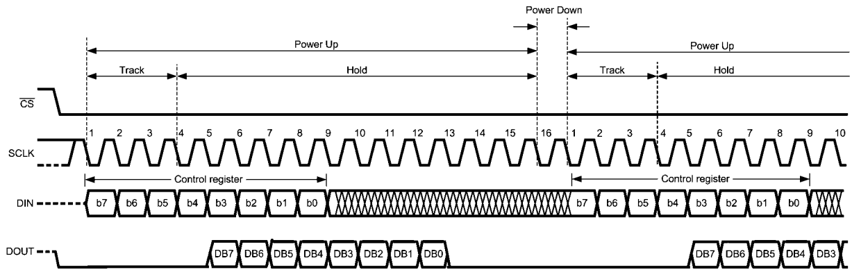
ADC084S051 Operational Timing Diagram
