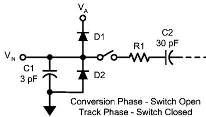
FIGURE 5. Equivalent Input Circuit
