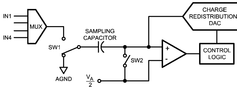
FIGURE 2. ADC084S051 in Hold Mode
